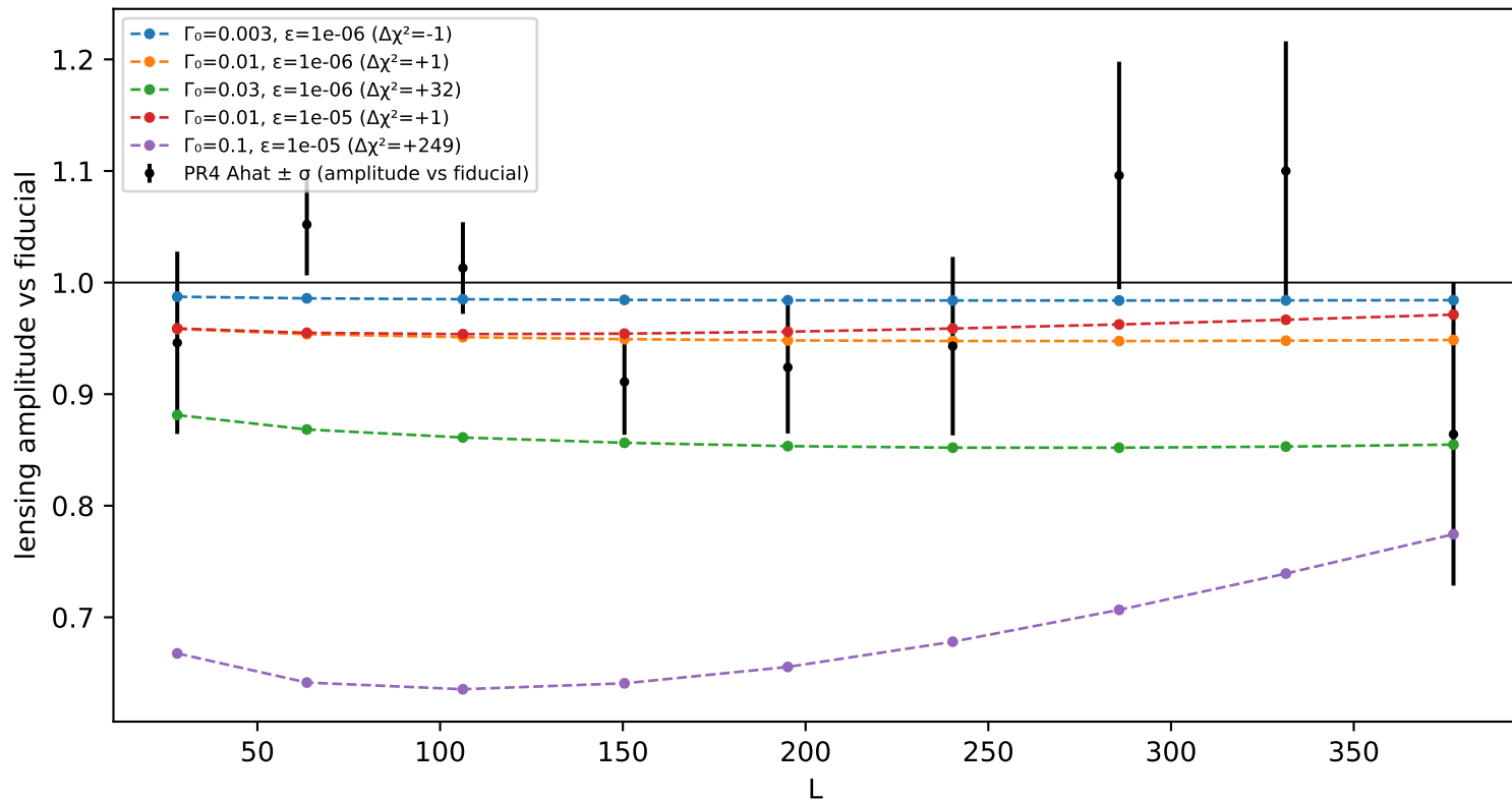
Planck PR4 lensing bandpowers vs guarded-CLASS suppression ( \nu -restored)
