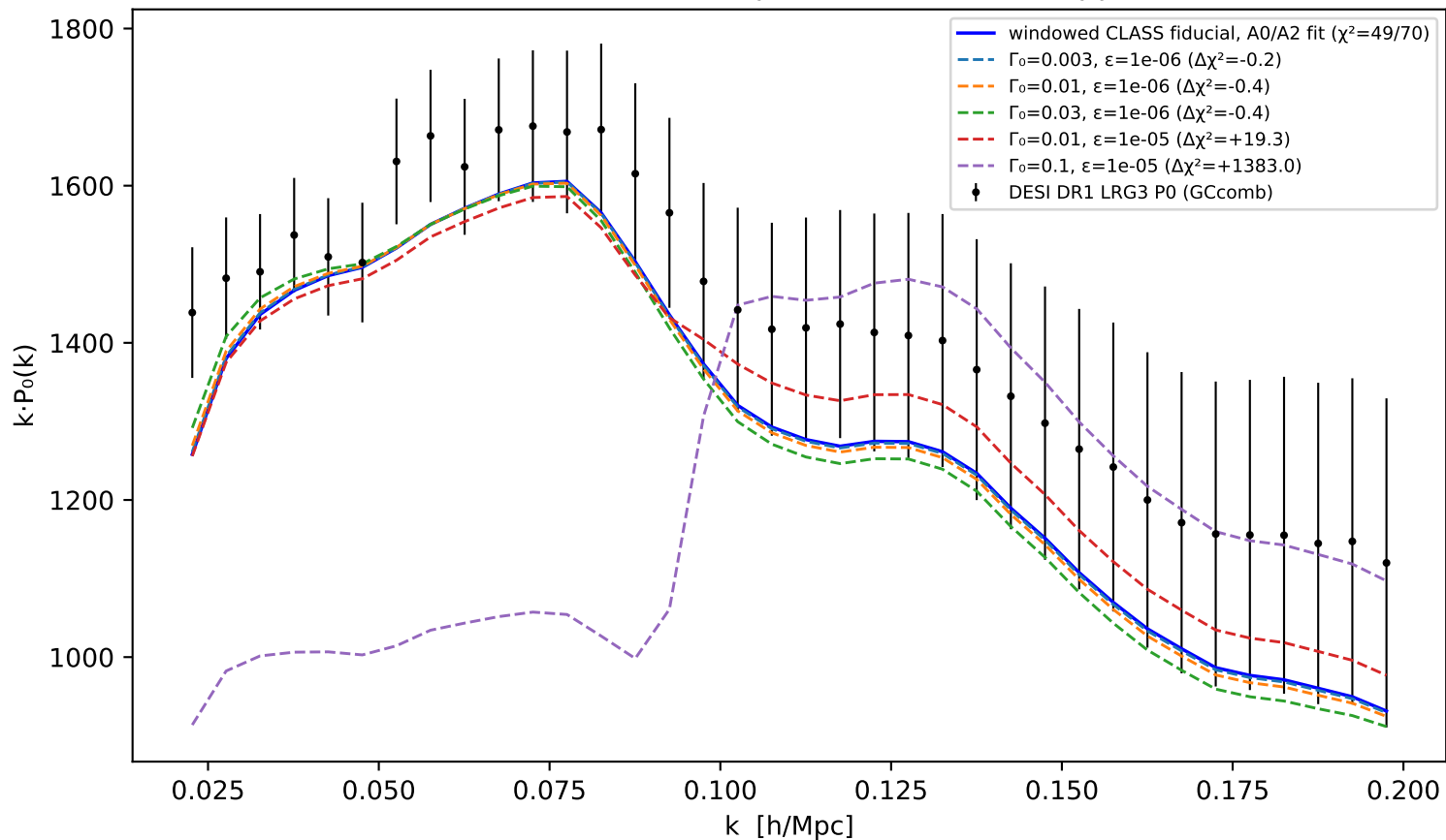
Tier-3 filter: DESI DR1 LRG3 monopole vs windowed suppression models
