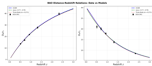
FIG. 6. BAO distance-redshift relations. Left: D_M/r_s . Right: D_H/r_s . The Three-Body modification (red dotted) shifts the predicted distances in the direction preferred by the DESI data (black points), with the effective H(z) enhancement of +0.5% at z = 0 growing to +1.1% at z = 1 .
