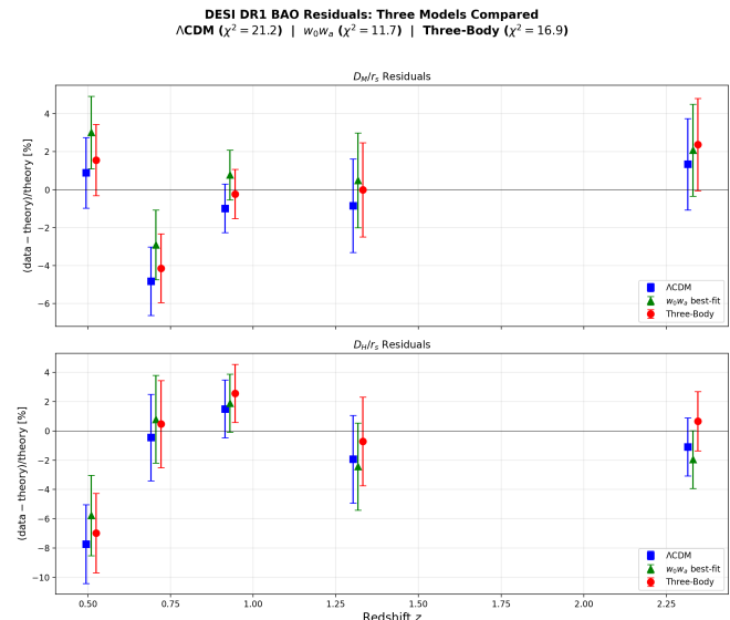
FIG. 5. DESI DR1 BAO residuals for all three models. Top : D_M/r_s residuals. Bottom : D_H/r_s residuals. The geometric friction model (red circles) consistently pulls the predictions toward the data at mid-redshift ( z \approx 0.5 – 1.3 ) compared to \Lambda\text{CDM} (blue squares), though the w_0w_a model (green triangles) achieves the tightest fit overall.
