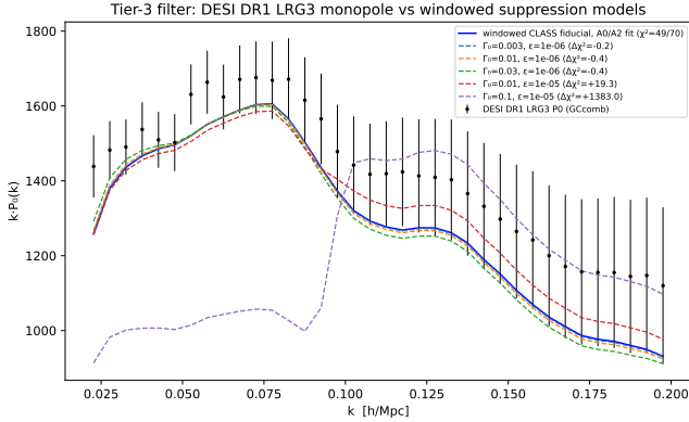
FIG. 3. DESI DR1 LRG ( 0.8 < z < 1.1 , GCcomb) monopole against window-convolved suppression models (amplitude-marginalized). The baseline fit ( \chi^2 = 48.9/70 ) validates the apparatus; the \epsilon = 10^{-5} family’s suppression edge inside the fitted window is unabsorbable, while the \epsilon \leq 10^{-6} family is degenerate with the bias amplitude.
