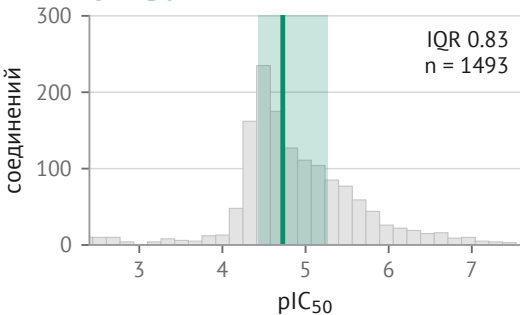
CYP2D6
