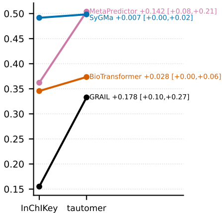
(b) external GLORYx ( n = 37 )
