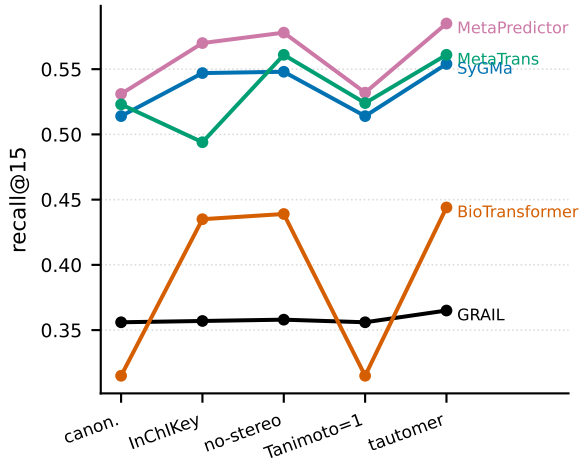
(a) internal ( n = 150 , 5 methods)
