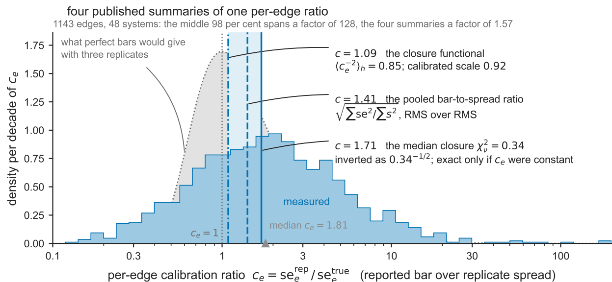
Figure 4: One heavy-tailed per-edge ratio, and the summaries this article quotes from it. The calibration ratio c_e = se_e^{\text{rep}} / se_e^{\text{true}} over the 1143 edges of the 48 systems that carry a cycle, on a logarithmic axis because c_e is a ratio, so a bar twice too wide and one twice too tight are equally miscalibrated, and because the tail is the reason the summaries disagree rather than a nuisance to be clipped. Quartiles 0.91, 1.81 and 3.60. Each mark is a different functional of this one distribution: the curl-leverage-weighted mean of c_e^{-2} that Theorem 1 makes \mathbb{E}[\chi^2_v] , together with its root the calibrated scale, which are one mark and not two; the replicate ratio of Figure 3, the pooled reported standard error over replicate spread, 1.41; and the inverted median, the median reduced \chi^2 of 0.34 inverted, which recovers a scalar conservatism only if c_e were constant across edges and carries that caveat on the figure. The grey silhouette is the distribution perfect bars would give at three replicates, where s^2/\sigma^2 \sim \chi^2_2/2 makes c_e = 1/\sqrt{\text{Exp}(1)} a parameter-free null with median 1.20: part of the measured spread is the denominator’s own small-sample noise and only the excess is per-edge heterogeneity. The panel adds no measurement, and no claim beyond the text’s: no single scalar conservatism is identified by these data. Reproduce with make figCal .
