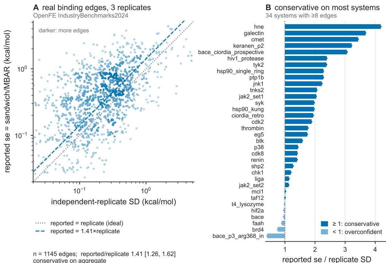
Figure 3: Independent-replicate validation on real binding edges. Reported per-edge standard error versus the across-replicate empirical standard deviation, on 1145 OpenFE IndustryBenchmarks2024 [2] edges (3 independent replicates each). (A) Reported standard error versus across-replicate standard deviation, with the y=x line. (B) Per-system pooled ratio of reported standard error to across-replicate standard deviation, for the 34 benchmark systems carrying at least eight edges.
