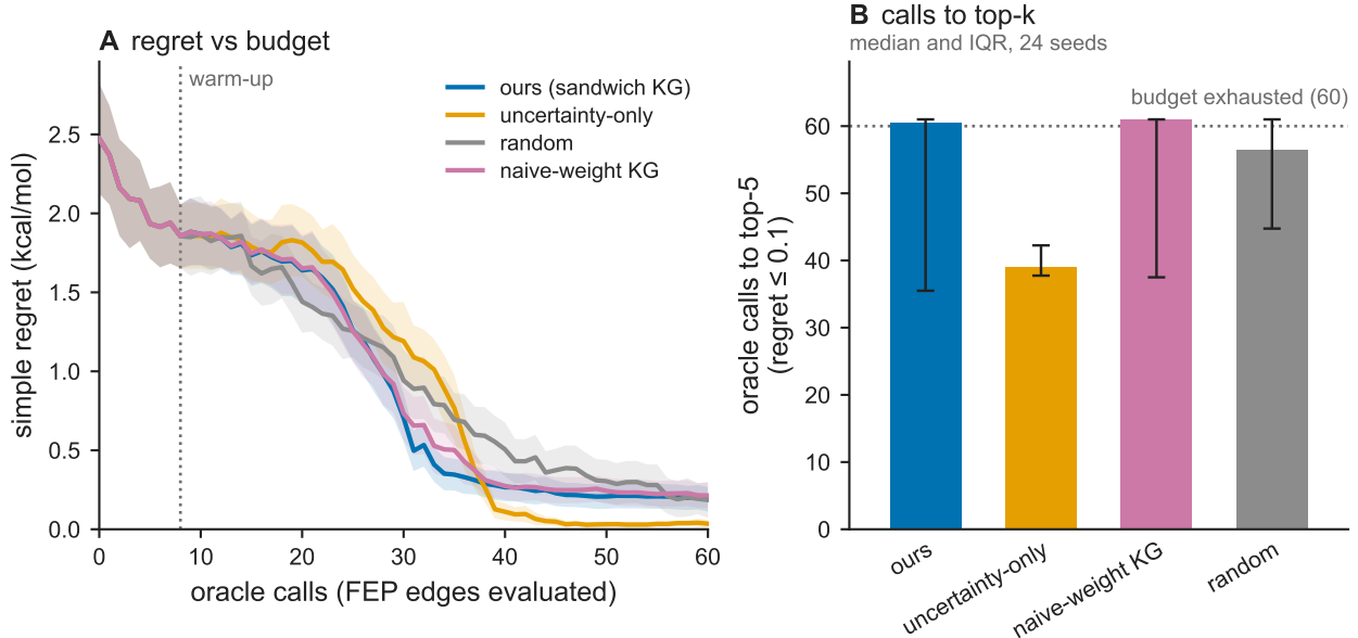
Figure S3: Simulated active-learning acquisition policies. (A) Simple regret versus oracle calls (simulated FEP edges evaluated), for a sandwich-weighted knowledge-gradient policy [8], implemented as in Balandat et al. [2] and Gardner et al. [9], a naive-weighted knowledge-gradient policy, an uncertainty-only policy, and random selection, averaged over 24 seeds with 95% confidence bands. (B) Median oracle calls to reach the top- k candidates (regret at or below tolerance), with interquartile-range error bars, for the same four policies.
