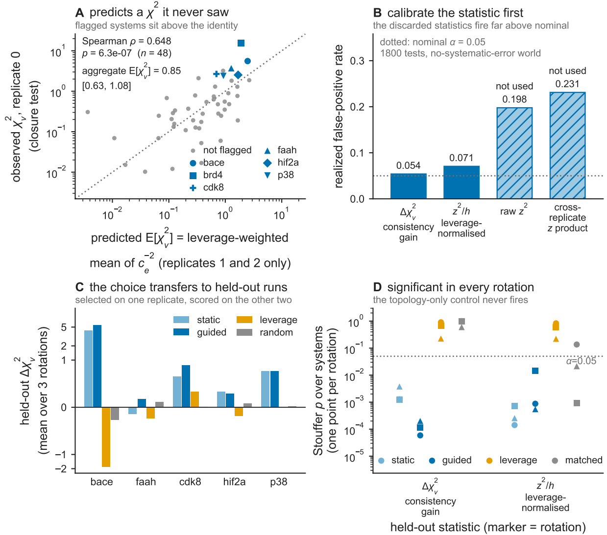
Figure S13: Out-of-sample behaviour of the calibrated null. (A) Per-system closure \chi_v^2 predicted from the per-edge miscalibration measured on the two replicates not being predicted, against the observed value, with the identity line and the flagged systems marked. (B) Realized false-positive rate of each candidate held-out statistic under a simulation with no systematic error anywhere, against the nominal level, with the two statistics that fire far above nominal marked. (C) Held-out change in reduced \chi^2 on the two replicates not used for selection, after removing the edges selected on the third, averaged over the three rotations and shown per testable flagged system, for a static and a guided selection rule, a topology-only rule built from curl-leverage, and equal-size random removal. (D) Stouffer-combined p -value over systems, one point per rotation, for each of the two statistics that held their nominal level, under the same selection rules together with an |z| -rank-matched control drawn from unflagged systems, with the \alpha = 0.05 line marked.
