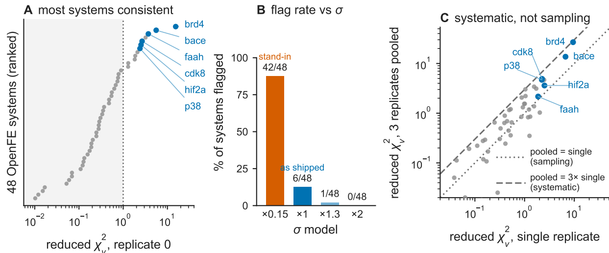
Figure 6: Calibrated cycle-closure quality control. (A) Per-system reduced \chi^2 from a generalized-least-squares cycle-closure fit, ranked, with shading below \chi^2_{\nu} = 1 and the flagged systems marked. (B) Percentage of systems flagged under four \sigma models, in plotted order: a uniform \times 0.15 shrink, the reported bar as shipped, a \times 1.3 inflation and a \times 2 inflation. The shipped bar is the tick marked \times 1 ; the scale at which those bars are correct is measured as 0.92 of them, which is a different quantity from the tick. (C) Reduced \chi^2 from a single replicate against the value from the three replicates pooled, with reference lines at pooled/single = 1 and = 3.
