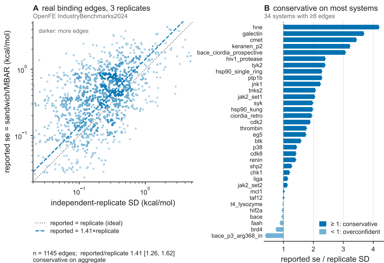
Figure 5: Independent-replicate validation on real binding edges. Reported per-edge standard error versus the across-replicate empirical standard deviation, on 1145 OpenFE IndustryBenchmarks2024 25 edges (3 independent replicates each). (A) Reported standard error versus across-replicate standard deviation, with the y=x line. (B) Per-system pooled ratio of reported standard error to across-replicate standard deviation, for the 34 benchmark systems carrying at least eight edges.
