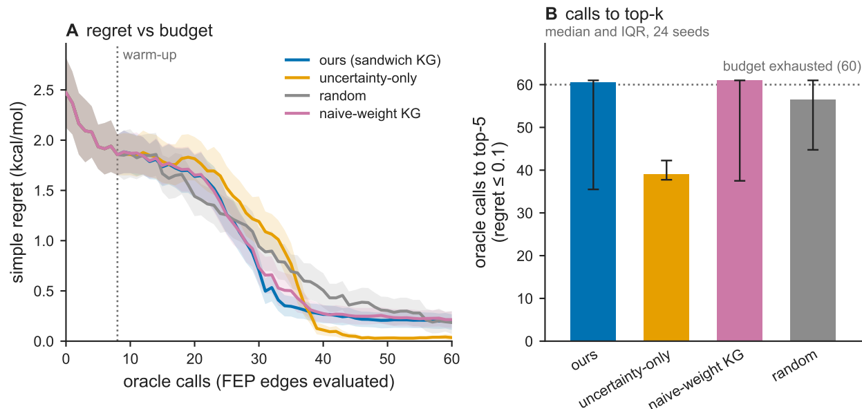
Figure S3: Simulated active-learning acquisition policies. (A) Simple regret versus oracle calls (simulated FEP edges evaluated), for a sandwich-weighted knowledge-gradient policy S9 , implemented as in Balandat et al. S10 and Gardner et al. S11 , a naive-weighted knowledge-gradient policy, an uncertainty-only policy, and random selection, averaged over 24 seeds with 95% confidence bands. (B) Median oracle calls to reach the top- k candidates (regret at or below tolerance), with interquartile-range error bars, for the same four policies.
