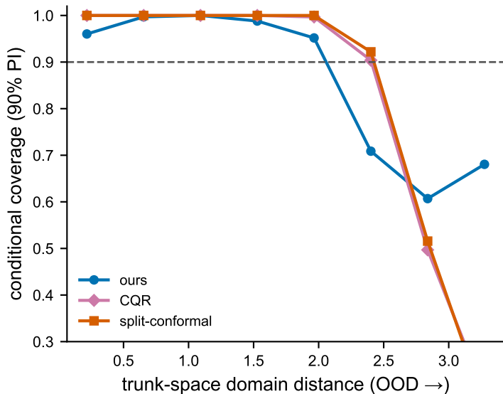
A coverage holds OOD vs conformal
