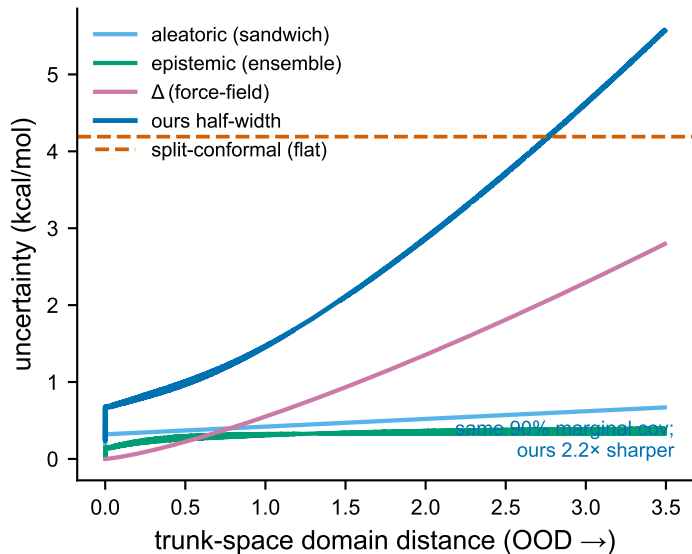
B decomposition: epistemic+ \Delta grow OOD
