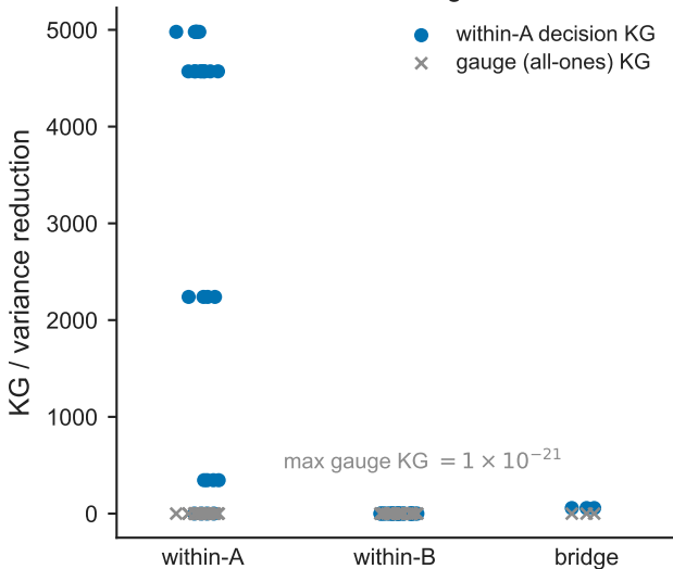
A KG routes to relevant edges
