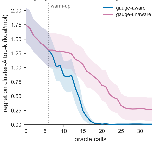
B gauge-awareness saves budget
