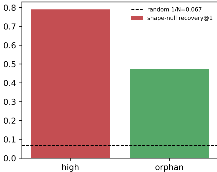
B shape-null collapse -> VALIDITY_KILL
