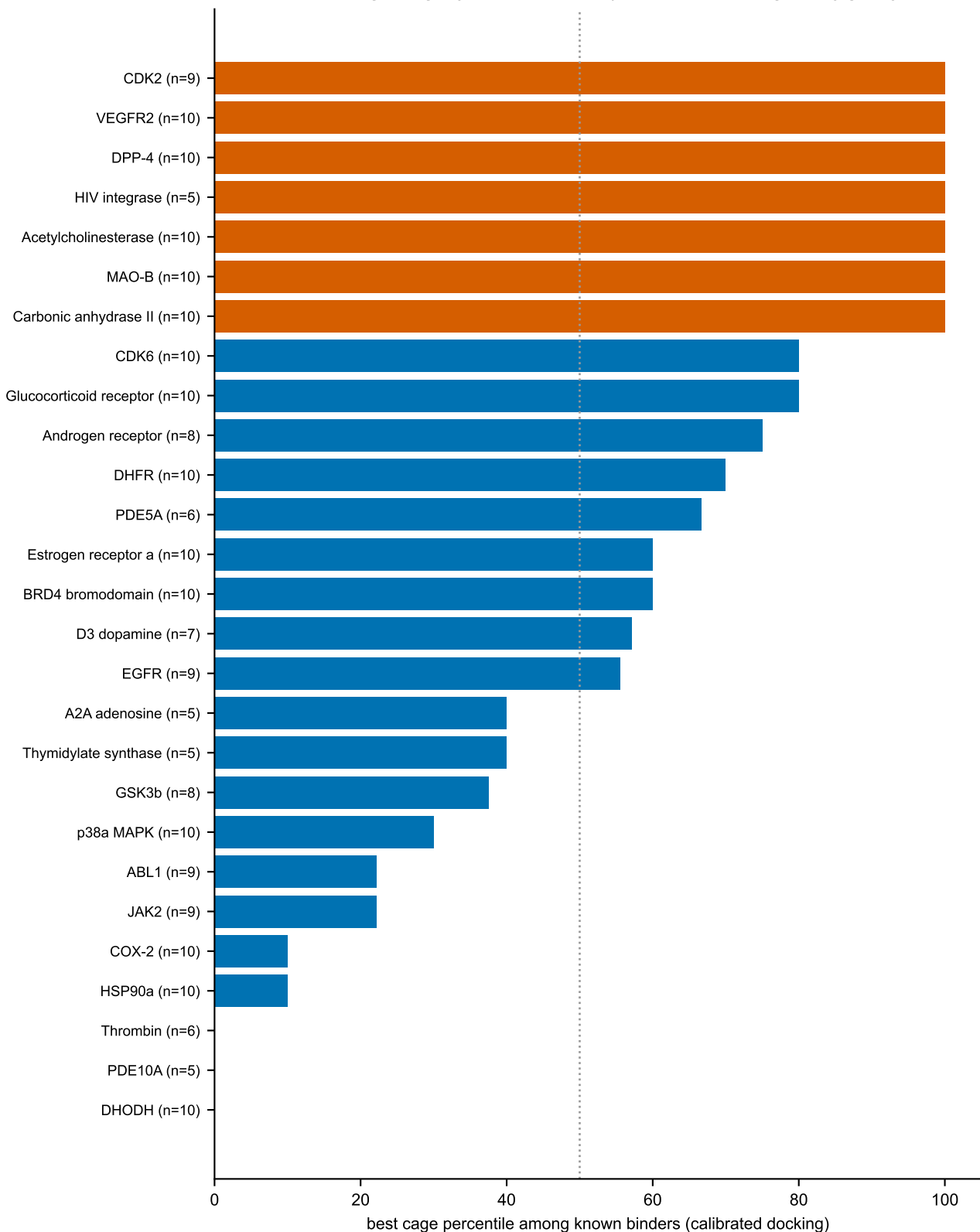
Calibrated reverse docking — cage hypothesis shortlist (PRELIMINARY; orange=likely greasy-pocket artefact)
