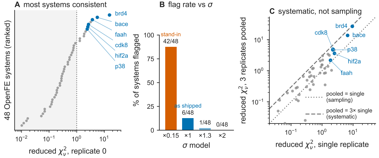
Figure 5: Calibrated cycle-closure quality control. (A) Per-system reduced \chi^2 from a generalized-least-squares cycle-closure fit, ranked, with shading below \chi^2_v = 1 and the flagged systems marked. (B) Percentage of systems flagged under four \sigma models, in plotted order: a uniform \times 0.15 shrink, the reported bar as shipped, a \times 1.3 inflation and a \times 2 inflation. The shipped bar is the tick marked \times 1 ; the scale at which those bars are correct is measured as 0.92 of them, which is a different quantity from the tick. (C) Reduced \chi^2 from a single replicate against the value from the three replicates pooled, with reference lines at pooled/single = 1 and = 3.
