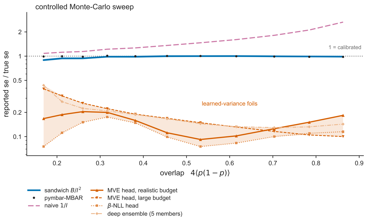
Figure S2: Reported standard error against the true standard error over a controlled overlap sweep. Reported standard error divided by the true standard error, versus work-distribution overlap, for the sandwich B/I^2 , pymbar-MBAR, the naive information-equality plug-in 1/I , a learned mean-variance (MVE) head at a realistic and at a large training budget, a \beta -NLL head, and a 5-member deep ensemble, in a controlled Monte-Carlo sweep.
