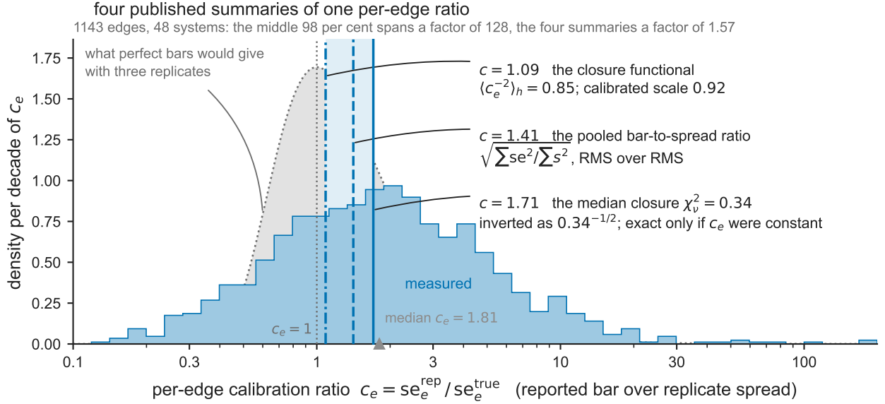
Figure 6: One heavy-tailed per-edge ratio, and the summaries this article quotes from it. The calibration ratio c_e = se_e^{\text{rep}} / se_e^{\text{true}} over the 1143 edges of the 48 systems that carry a cycle, on a logarithmic axis because c_e is a ratio, so a bar twice too wide and one twice too tight are equally miscalibrated, and because the tail is the reason the summaries disagree rather than a nuisance to be clipped. Quartiles 0.91, 1.81 and 3.60. Each mark is a different functional of this one distribution: the curl-leverage-weighted mean of c_e^{-2} that Theorem 1 makes \mathbb{E}[\chi^2_\nu] , together with its root the calibrated scale, which are one mark and not two; the replicate ratio of Figure 5, the pooled reported standard error over replicate spread, 1.41; and the inverted median, the median reduced \chi^2 of 0.34 inverted, which recovers a scalar conservatism only if c_e were constant across edges and carries that caveat on the figure. The grey silhouette is the distribution perfect bars would give at three replicates, where s^2/\sigma^2 \sim \chi^2_2/2 makes c_e = 1/\sqrt{\text{Exp}(1)} a parameter-free null with median 1.20: part of the measured spread is the denominator’s own small-sample noise and only the excess is per-edge heterogeneity. The panel adds no measurement, and no claim beyond the text’s: no single scalar conservatism is identified by these data. Reproduce with make figCal .
