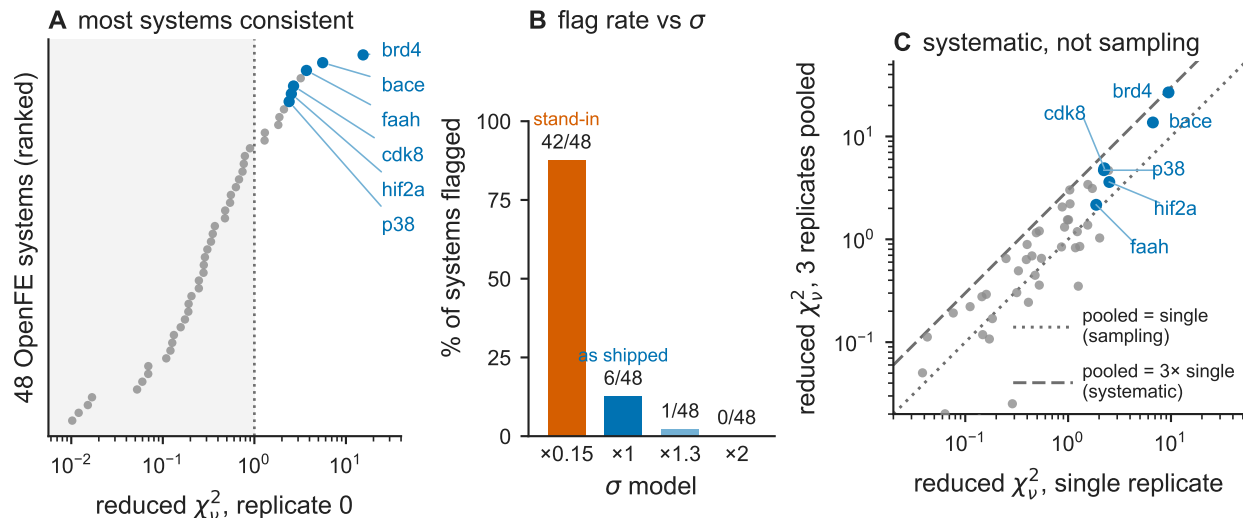
Figure 7: Calibrated cycle-closure quality control. (A) Per-system reduced \chi^2 from a generalized-least-squares cycle-closure fit, ranked, with shading below \chi^2_v = 1 and the flagged systems marked. (B) Percentage of systems flagged under four \sigma models, in plotted order: a uniform \times 0.15 shrink, the reported bar as shipped, a \times 1.3 inflation and a \times 2 inflation. The shipped bar is the tick marked \times 1 ; the scale at which those bars are correct is measured as 0.92 of them, which is a different quantity from the tick. (C) Reduced \chi^2 from a single replicate against the value from the three replicates pooled, with reference lines at pooled/single = 1 and = 3.
