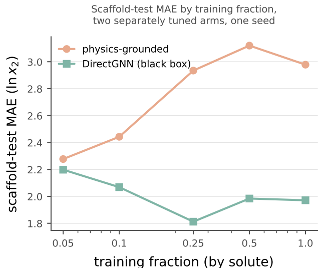
Figure S5: Data-efficiency curve: scaffold-test MAE of the physics-grounded arm (salmon) and of DirectGNN (teal) at five training-data fractions, one seed. The plotted values are the MAE columns of Table S25.
