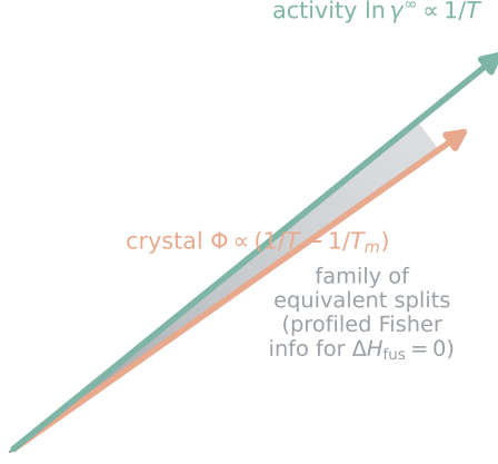
Figure 3: Why the crystal/activity split is non-identifiable from solubility. (a) As functions of 1/T the crystal direction \Phi and the activity direction \ln \gamma^\infty are nearly collinear, so a whole band of crystal/activity splits fits the data equally well (the profiled Fisher information for \Delta H_{\text{fus}} is zero, Lemma 1). (b) An external single-component label points off that axis and collapses the band to a point, pinning the split—the mechanism behind the aux-stream grounding, with the measured Cramér–Rao drop on \Delta H_{\text{fus}} .
