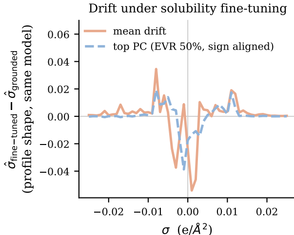
Figure 3: The drift solubility fine-tuning imposes on the learned \sigma -profile ( n=44 VT-2005-matched molecules): \hat{\sigma} after fine-tuning minus the same model’s grounded profile , not minus the external reference. Shown are the mean drift and its dominant PCA mode, defined only up to sign and drawn in the mean drift’s direction. Its spectrum, the null it lacks and the controls: §6.4, §E.
