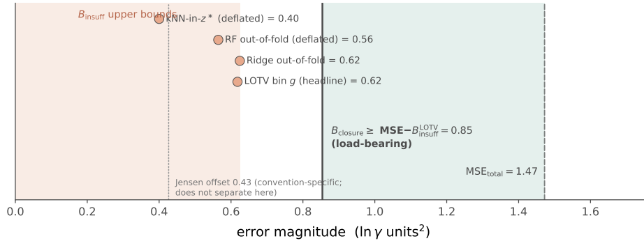
Figure 7: One-sided bounds on the closure-insufficiency split under the deployed residual-only COSMO-SAC convention—the configuration the model actually runs. The load-bearing, convention-independent bound B_{\text{closure}} \geq \text{MSE} - B_{\text{insuff}}^{\text{LOTV}} \approx 0.85 exceeds every valid B_{\text{insuff}} upper bound (salmon region); the white gap is a separation that needs no smoothness assumption, and the teal region is the certified closure share of the total error ( \text{MSE} = 1.47 ). We headline the law-of-total-variance (LOTV) binning bound because it conditions on the scalar g(z^*) and is immune to the near-duplicate leakage that deflates the z^* -neighbour estimators ( k -NN, RF; §6.2). The assumption-free Jensen constant-offset bound is convention-specific and inverts here ( 0.43 < 0.62 , dotted), which is why we do not lean on it.
