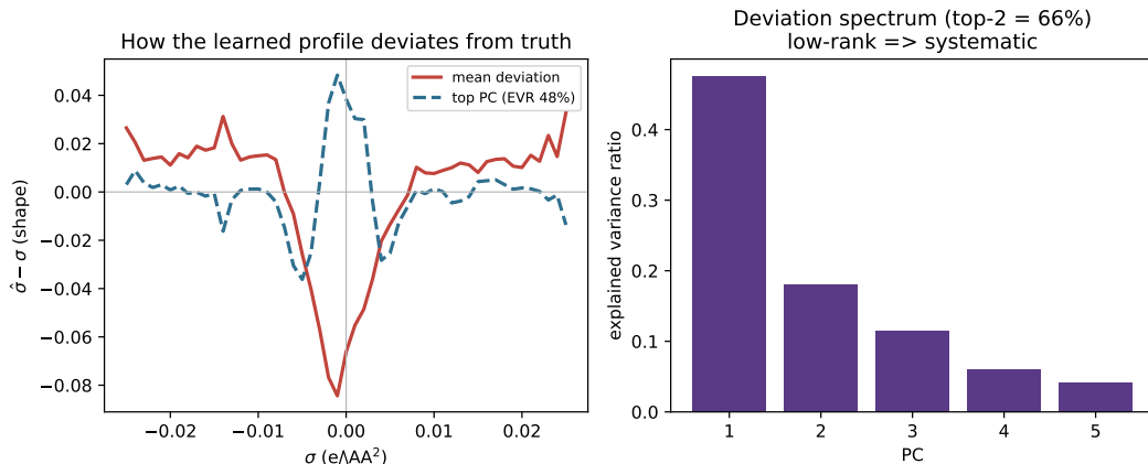
Figure 8: The learned \sigma -profile is a systematic closure-compensating surrogate, not the physical profile. Left: the mean deviation \hat{\sigma} - \sigma (and its dominant PCA mode) transfers area out of the nonpolar bins ( \sigma \approx 0 ) into the polar wings—the network makes molecules look more polar than they are, inflating the segment interactions the misspecified closure under-weights. Right: the deviation spectrum is low-rank (top-two modes 66%; noise would be flat at \approx 4\% ), i.e. the distortion is systematic. A single affine distortion transfers 16\times better than identity out-of-sample, so \hat{\sigma} is a transferable closure-inverse of \sigma , not \sigma with noise ( n=44 matched VT-2005 molecules).
