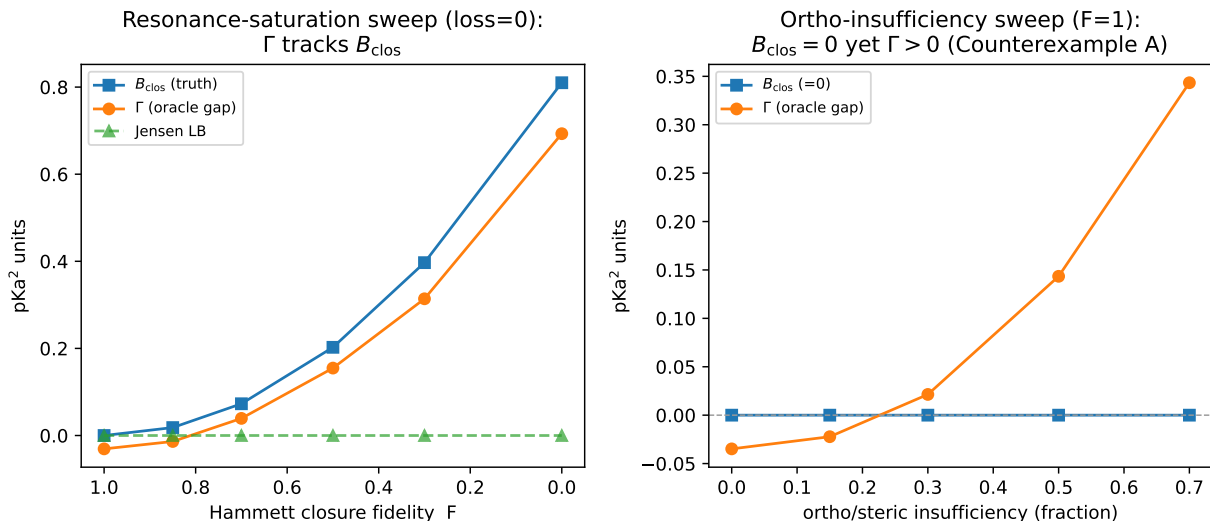
Figure 15: The diagnostic transfers to a second real closure (pKa through a Hammett LFER), on a controlled construction with known ground-truth channels. Left : varying closure fidelity with a sufficient intermediate, the grounding gap \Gamma tracks the closure bias B_{\text{closure}} (the assumption-light Jensen bound is flat here because the misspecification carries no mean offset). Right : varying an ortho/steric insufficiency channel with a well-specified closure, B_{\text{closure}} = 0 throughout while \Gamma > 0 grows—the pKa realization of the two-cause conflation of §4.3, and the reason certification rests on the decomposition, not on \Gamma .
