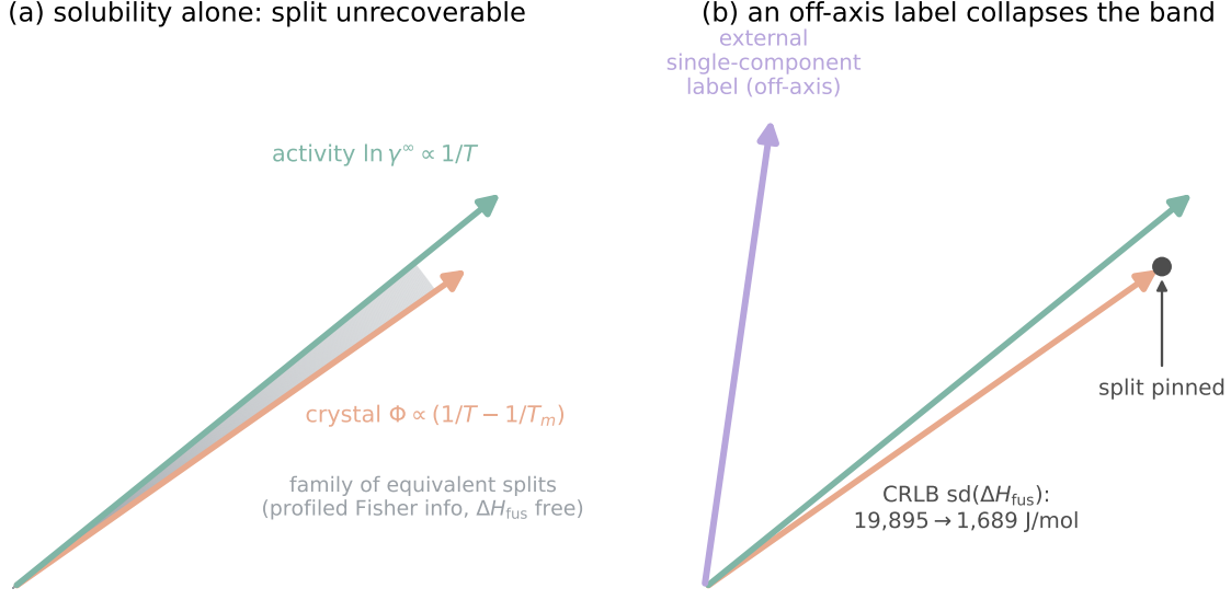
Figure 4: Why the crystal/activity split is non-identifiable from solubility. (a) As functions of 1/T the crystal direction \Phi and the activity direction \ln \gamma^\infty are nearly collinear, so a whole band of crystal/activity splits fits the data equally well (the profiled Fisher information for \Delta H_{\text{fus}} is zero, Lemma 1). (b) An external single-component label points off that axis and collapses the band to a point, pinning the split—the mechanism behind the aux-stream grounding, with the measured Cramér–Rao drop on \Delta H_{\text{fus}} .
