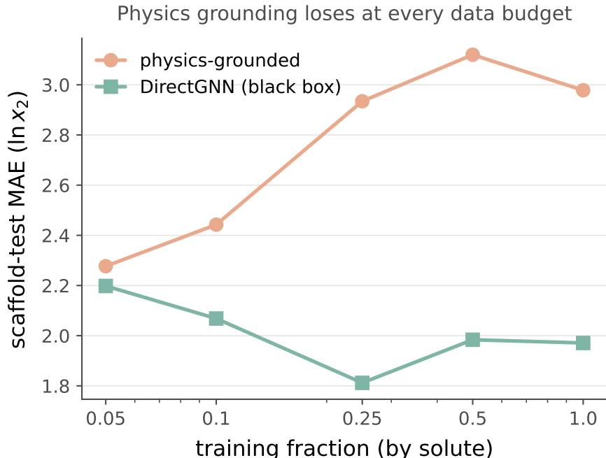
Figure 12: Data-efficiency curve. The physics-grounded arm (salmon) trails the DirectGNN black box (teal) at every training-data fraction; the gap is smallest at the least data and large thereafter—the opposite of the low-data advantage a physics prior is supposed to provide.
