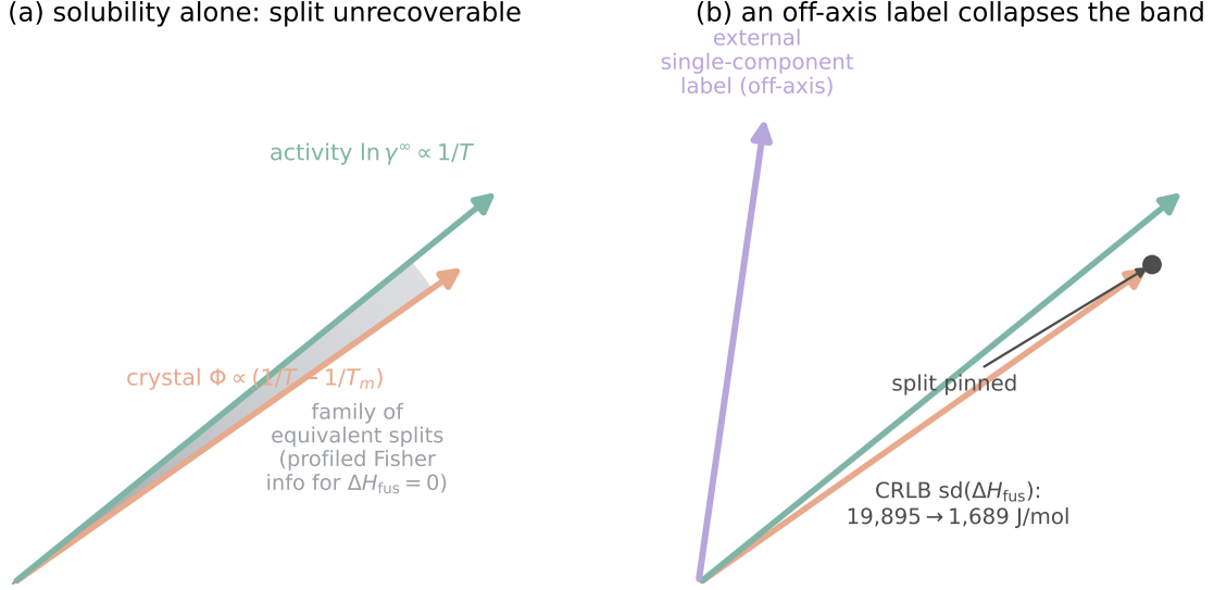
Figure 3: Why the crystal/activity split is non-identifiable from solubility. (a) As functions of 1/T the crystal direction \Phi and the activity direction \ln \gamma^\infty are nearly collinear, so a whole band of crystal/activity splits fits the data equally well (the profiled Fisher information for \Delta H_{\text{fus}} is zero, Lemma 1). (b) An external single-component label points off that axis and collapses the band to a point, pinning the split—the mechanism behind the aux-stream grounding, with the measured Cramér–Rao drop on \Delta H_{\text{fus}} .
