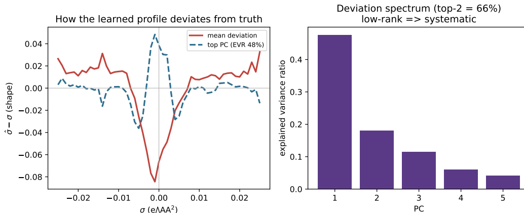
Figure 8: The learned \sigma -profile is a systematic closure-compensating surrogate, not the physical profile. Left : the mean deviation \hat{\sigma} - \sigma (and its dominant PCA mode) transfers area out of the nonpolar bins ( \sigma \approx 0 ) into the polar wings—the network makes molecules look more polar than they are, inflating the segment interactions the misspecified closure under-weights. Right : the deviation spectrum is low-rank (top-two modes 66%; noise would be flat at \approx 4\% ), i.e. the distortion is systematic. A single affine distortion transfers 16\times better than identity out-of-sample, so \hat{\sigma} is a transferable closure-inverse of \sigma , not \sigma with noise ( n=44 matched VT-2005 molecules).
