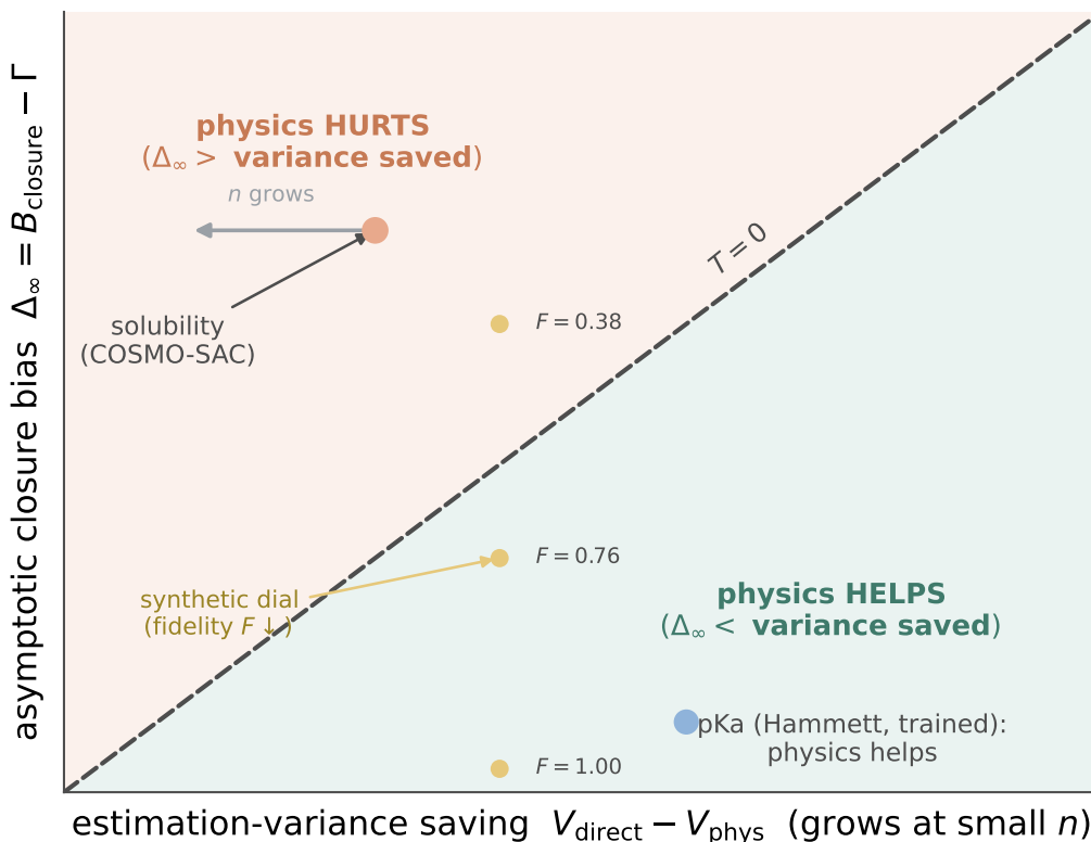
Figure 13: When a physics prior helps versus hurts. The physics tax has sign \mathcal{T} = \Delta_\infty - (variance saved): a fixed-closure prior helps only below the \mathcal{T} = 0 diagonal, where the estimation variance it saves exceeds its asymptotic closure bias \Delta_\infty (the large- n asymptote; = B_{\text{closure}} - \Gamma under A2). The variance saving shrinks as n grows, so systems drift left: solubility/COSMO-SAC sits deep in the “hurts” region and moves further in with more data, pKa through a Hammett closure lands on the “physics helps” side as a trained comparison (§6.6)—though a stratified check shows the help is not cleanly a closure-fidelity effect—and the synthetic dial climbs out of “helps” as closure fidelity F falls. Conceptual—only the sign is measured, not the boundary’s exact shape.
