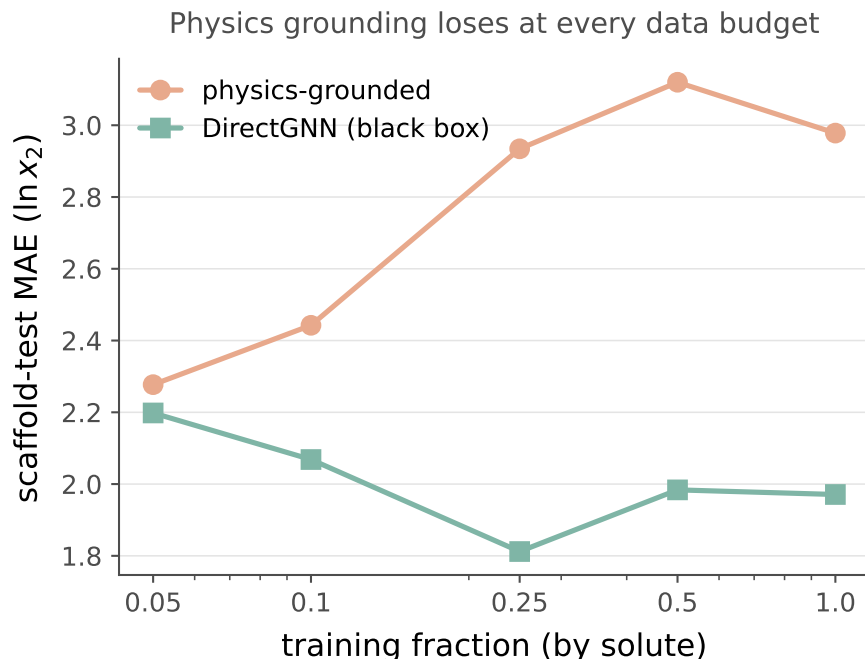
Figure 13: Data-efficiency curve. The physics-grounded arm (salmon) trails the DirectGNN black box (teal) at every training-data fraction; the gap is smallest at the least data and large thereafter—the opposite of the low-data advantage a physics prior is supposed to provide.
