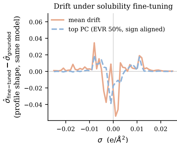
Figure S5: The drift solubility fine-tuning imposes on the learned \sigma -profile ( n=44 VT-2005-matched molecules): \hat{\sigma} after fine-tuning minus the same model’s grounded profile , not minus the external reference. Shown are the mean drift and its dominant PCA mode, defined only up to sign and drawn in the mean drift’s direction; the legend’s EVR is that mode’s explained variance ratio.
