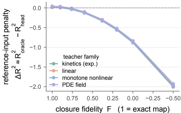
Reference-input penalty against closure fidelity (four synthetic teacher families, six misspecification forms)
