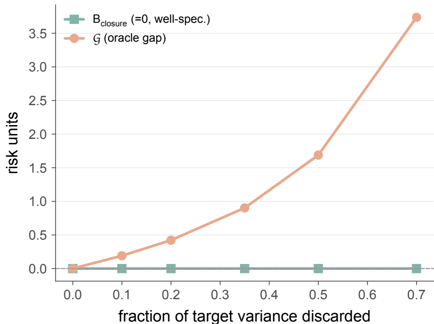
A2 violated, closure well-specified: B_{\text{closure}} = 0 yet \mathcal{G} > 0
