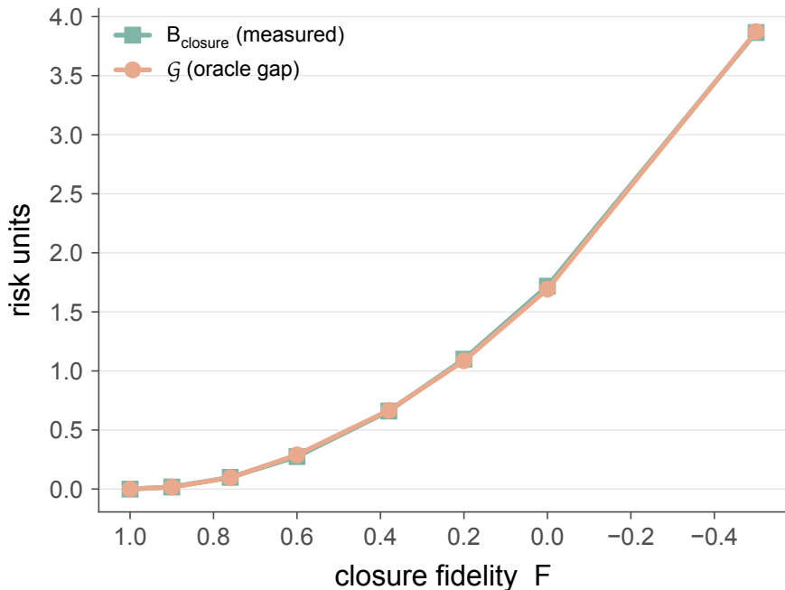
A2 holds: \mathcal{G} tracks B_{\text{closure}} ( \mathcal{G} is a valid proxy)
