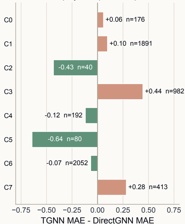
Where the physics path helps or hurts
