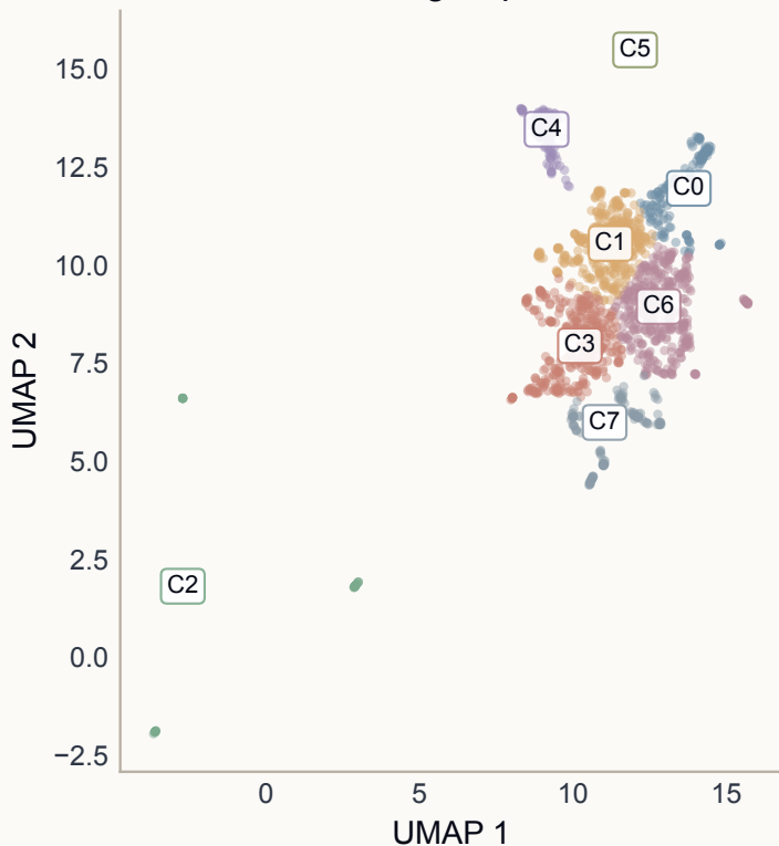
Functional-group clusters
