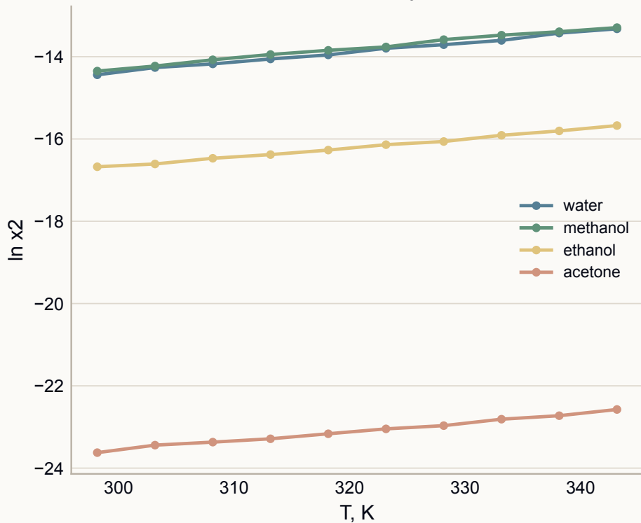
Delphinidin chloride: measured solubility curves
