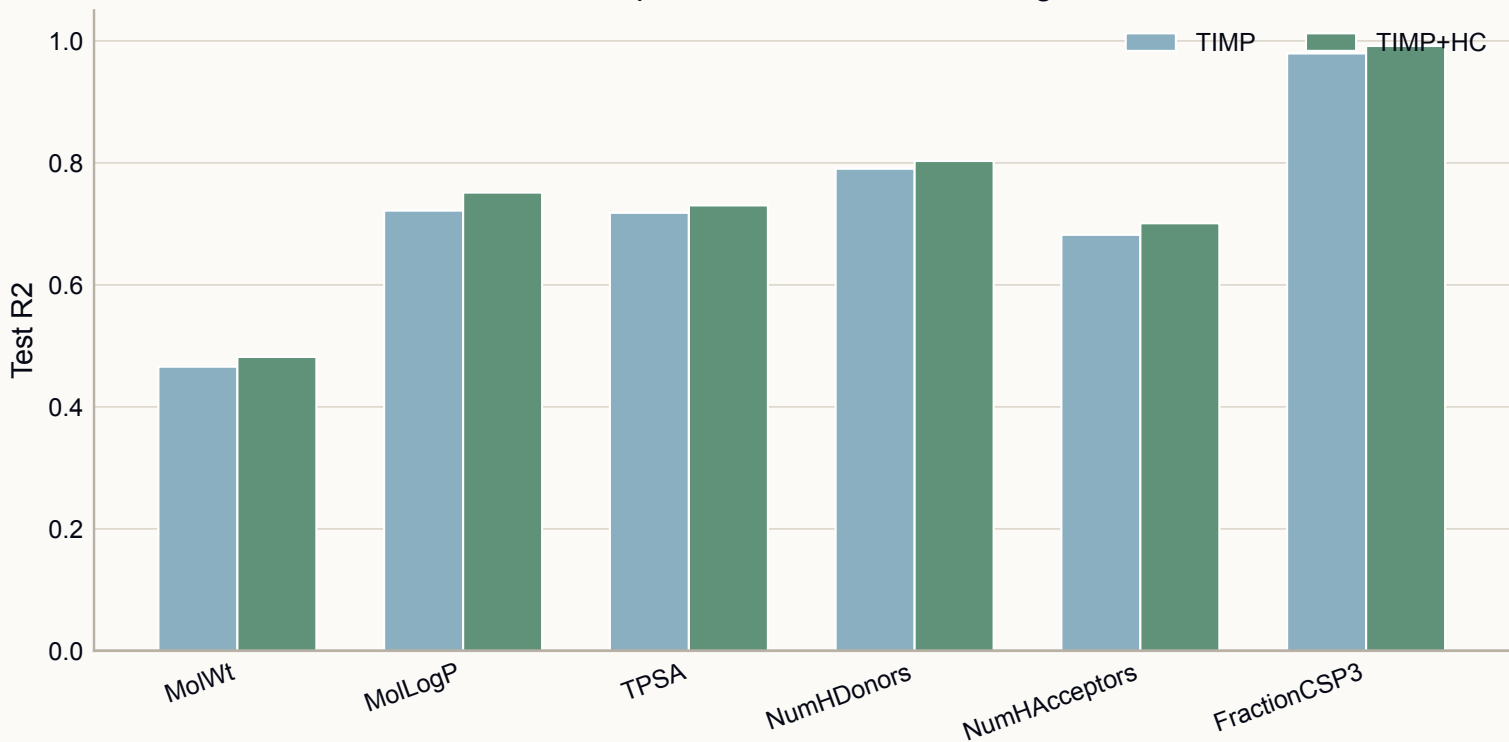
Linear probe on frozen embeddings
