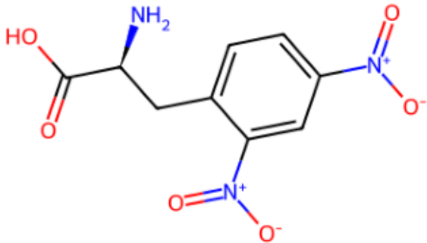
2,4-dinitro-L-phenylalanine
