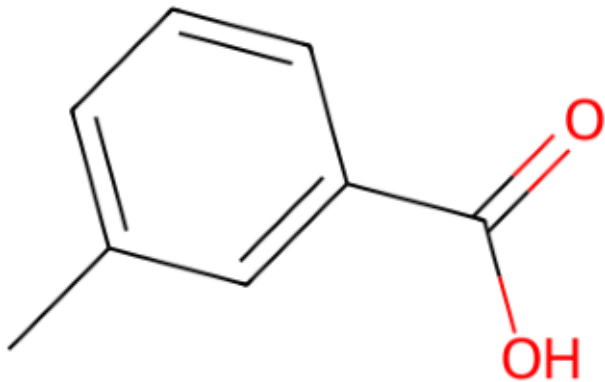
m-methylbenzoic acid
