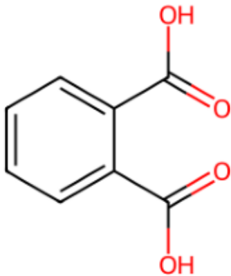
o-phthalic acid
