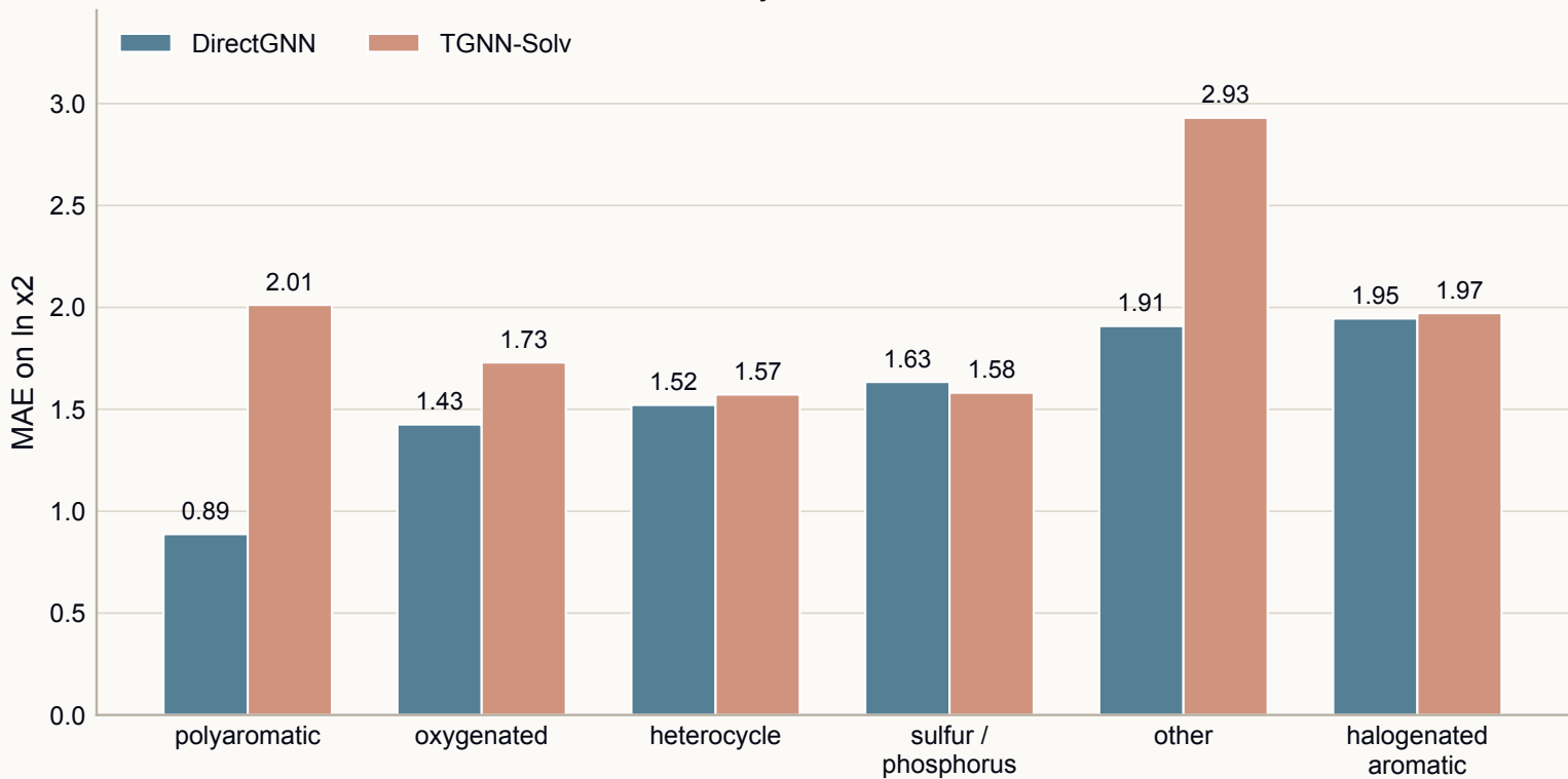
Error by chemical class
