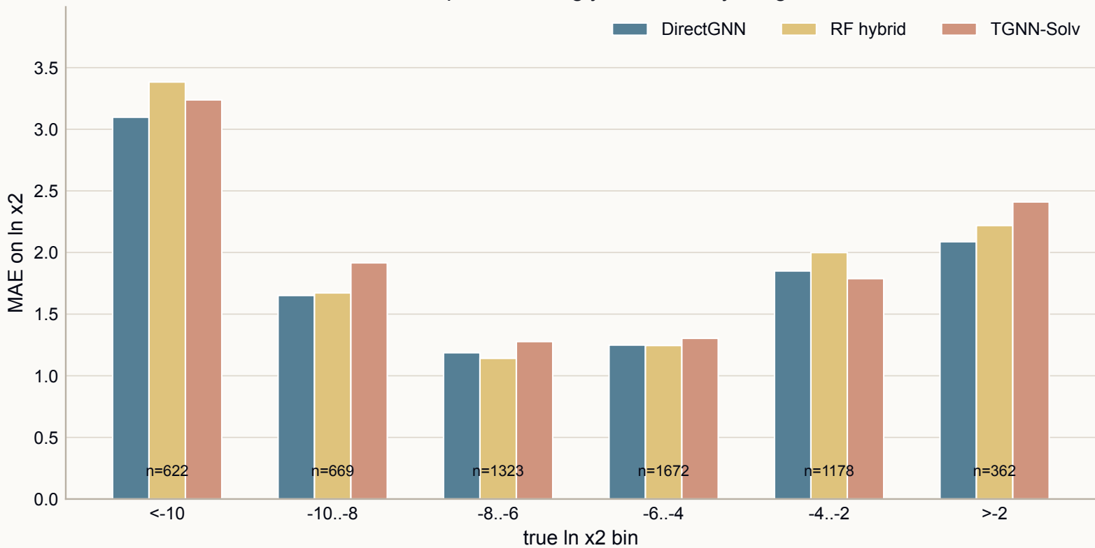
Error depends strongly on solubility range
