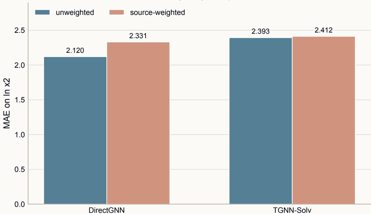
Source weighting proxy ablation
