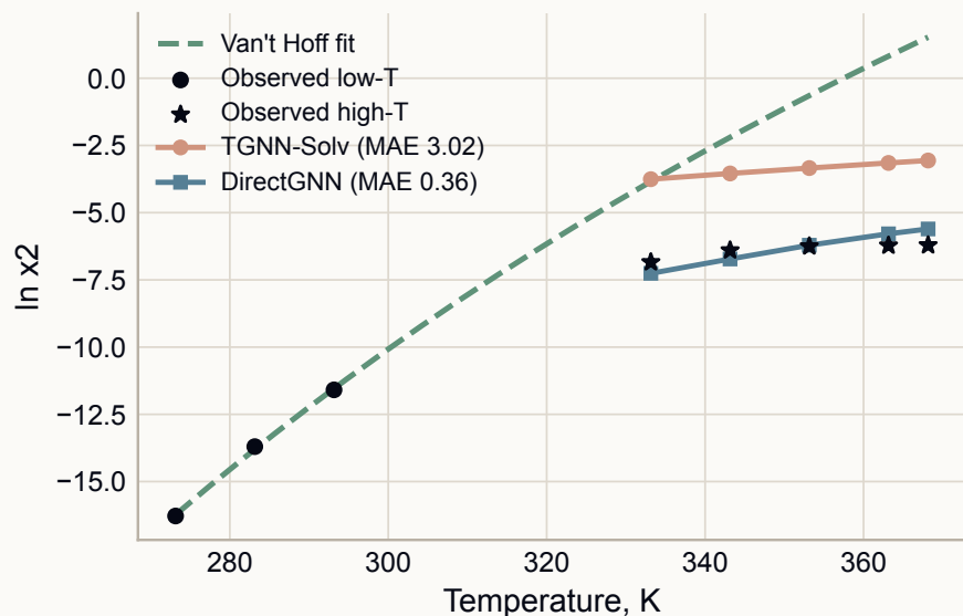
Very low-solubility tail Delphinidin ethanol
