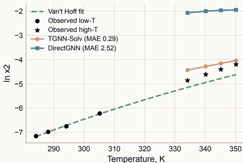
Large activity correction needed Delphinidin acetone
