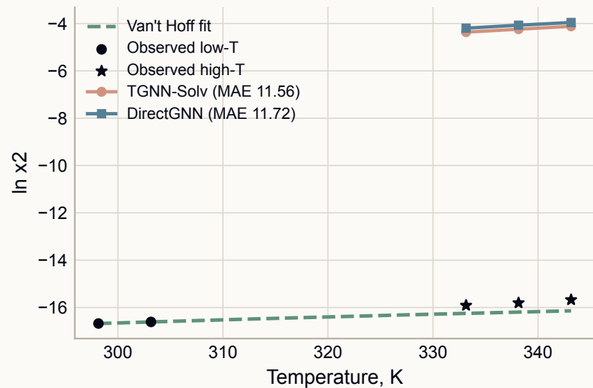
Very low-solubility tail Delphinidin ethanol
