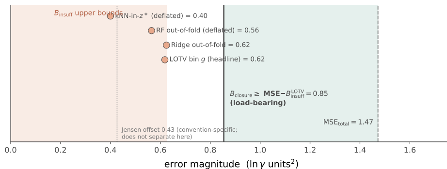
Figure 8: One-sided bounds on the closure-insufficiency split under the deployed residual-only COSMO-SAC convention—the configuration the model actually runs. The load-bearing, convention-independent bound B_{\text{closure}} \geq \text{MSE} - B_{\text{insuff}}^{\text{LOTV}} \approx 0.85 exceeds every valid B_{\text{insuff}} upper bound (salmon region); the white gap is a separation that needs no smoothness assumption, and the teal region is the certified closure share of the total error ( \text{MSE} = 1.47 ). We headline the law-of-total-variance (LOTV) binning bound because it conditions on the scalar g(z^*) and is immune to the near-duplicate leakage that deflates the z^* -neighbour estimators ( k -NN, RF; §6.2). The assumption-free Jensen constant-offset bound is convention-specific and inverts here ( 0.43 < 0.62 , dotted), which is why we do not lean on it.
