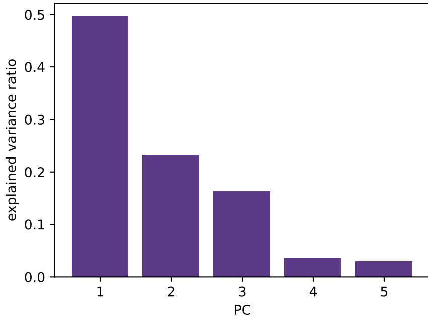
Deviation spectrum (top-2 = 73%) low-rank => systematic
