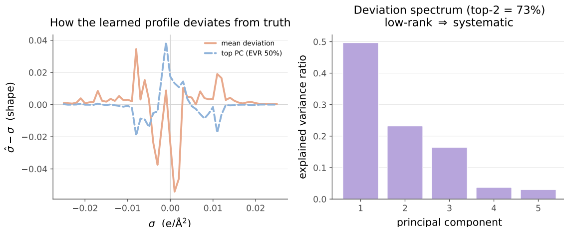
Figure 4: The learned \sigma -profile is a systematic closure-compensating surrogate, not the physical profile. Left : the mean deviation \hat{\sigma} - \sigma (and its dominant PCA mode) transfers area out of the nonpolar bins ( \sigma \approx 0 ) into the polar wings—the network makes molecules look more polar than they are, inflating the segment interactions the misspecified closure under-weights. Right : the deviation spectrum is low-rank (top-two modes 72 \pm 1\% , 4.8\times the finite-sample isotropic null of \approx 15\% at n=44 , p=51 ), i.e. the distortion is systematic. A single ridge-fit affine distortion (2652 parameters, 22 train / 22 held out) transfers 4.1 \pm 0.5\times better than the zero-drift null out-of-sample (spectrum mean-removed), so \hat{\sigma} is a transferable closure-compensating surrogate of \sigma , not \sigma with noise (confound-free, three seeds, n=44 matched VT-2005 molecules).
