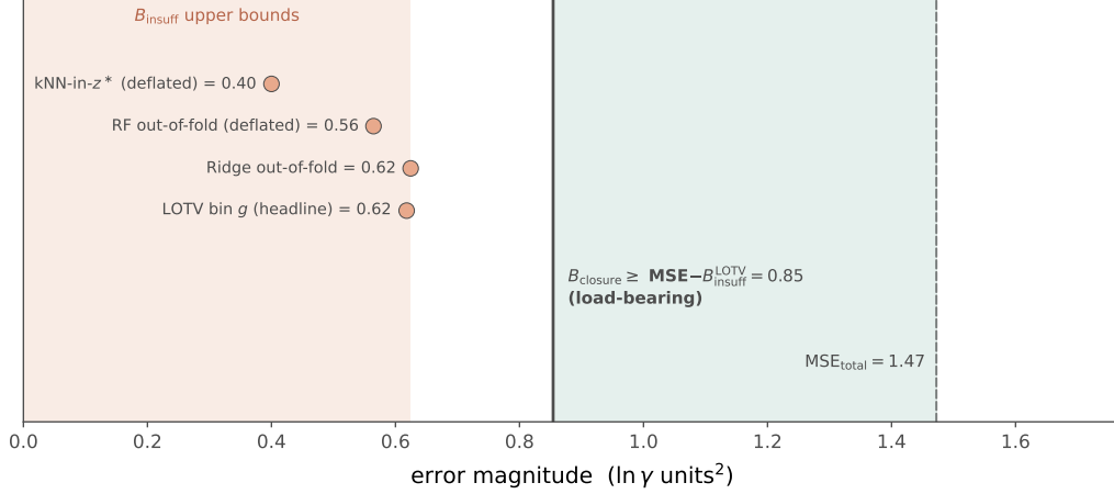
Figure 3: One-sided bounds on the closure-insufficiency split under the deployed residual-only COSMO-SAC convention—the configuration the model actually runs. The load-bearing, convention-independent bound B_{\text{closure}} \geq \text{MSE} - B_{\text{insuff}}^{\text{LOTV}} \approx 0.85 exceeds every valid B_{\text{insuff}} upper bound (salmon region); the white gap is a separation that needs no smoothness assumption, and the teal region is the closure share of the total error lower-bounded by that margin (deterministic on this n=60 set; its generalization is the two-way cluster-bootstrap frequency P_{\text{boot}} \approx 0.78 ) ( \text{MSE} = 1.47 ). We headline the law-of-total-variance (LOTV) binning bound because it conditions on the scalar g(z^*) and is immune to the near-duplicate leakage that deflates the z^* -neighbour estimators ( k -NN, RF; §6.2). The convention-specific constant-offset (Jensen) bound inverts under this deployed convention; its numbers are reported with the convention hedge in App. C.
