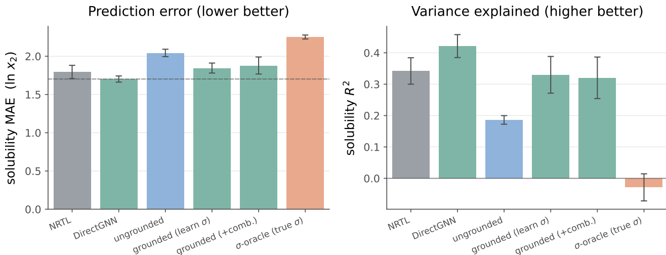
Figure 2: Controlled comparison on the scaffold split (3 seeds, mean \pm sd, n=5608 ; metrics are the 3-seed mean of the cross-arm intersection lock, over rows supervised and finite in every arm). DirectGNN shares the encoder but has no thermodynamic closure; the physics closures trail it (the asymptotic physics penalty). Replacing the model’s learned \sigma -profile with the reference VT-2005 profile (the \sigma -oracle, salmon) gives the worst arm, collapsing R^2 to \approx 0 ( -0.03 \pm 0.04 ): by MAE the model predicts solubility distinctly better from its invented \sigma (1.85) than from the reference one (2.25). This is the paper’s motivating symptom : because few drug-like solutes have a reference profile, the substitution here lands almost entirely on the solvent, so the closure-versus-input attribution is carried on the clean activity axis (§6.2, §6.4), not on this panel. Per-arm exact values are transcribed in the SI.
