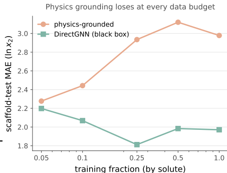
Figure 8: Data-efficiency curve. The physics-grounded arm (salmon) trails the DirectGNN black box (teal) at every training-data fraction; the gap is smallest at the least data and large thereafter—the opposite of the low-data advantage a physics prior is supposed to provide.
