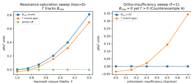
Figure 9: The diagnostic transfers to a second real closure (pKa through a Hammett LFER), on a controlled construction with known ground-truth channels. Left : varying closure fidelity with a sufficient intermediate, the grounding gap \Gamma tracks the closure bias B_{\text{closure}} (the assumption-light Jensen bound is flat here because the misspecification carries no mean offset). Right : varying an ortho/steric insufficiency channel with a well-specified closure, B_{\text{closure}} = 0 throughout while \Gamma > 0 grows—the pKa realization of the two-cause conflation of §4.3, and the reason certification rests on the decomposition, not on \Gamma .
