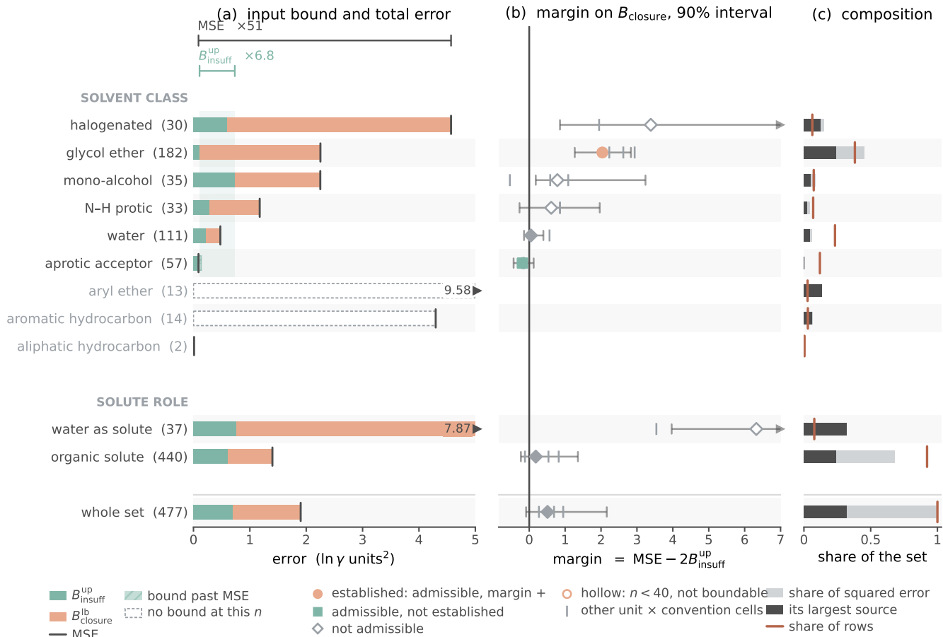
Figure 5: Where the closure binds, and where it is not established , by solvent class and by solute role, on the broad IDAC set (477 rows, 185 pairs, 78 solutes, 36 solvents, 15 source publications). Bars, points and shares are at the row unit under the deployed residual-only convention, at one estimator cell for every stratum—eight equal-count bins of g(z^*) with the Bessel within-bin variance. (a) each stratum’s input-insufficiency bound and its total error; (b) the margin between them with its 90% two-way cluster-bootstrap interval, the other three unit \times convention cells as grey ticks; (c) each stratum’s share of the set’s squared error, the part carried by its largest source publication drawn dark. This is the drawn form of the twelve cells at the reported granularity; the map itself, all 59 strata with their sources, intervals and admissibility, is Tables 3 and 4 in the main text. The marker in (b) is the admissibility verdict of §4.2(i), read off the same deposited columns the tables are built from. Grade: likely for the glycol ethers, the one row set of the map’s six admissible cells that is both positive and not contained in another, here at P > 0.95 ; open for every other row, the aggregate included. Caveat: a hollow marker is a stratum below n=40 —four of the drawn cells, with margins +0.78 , +0.61 , +3.39 and +6.33 , none of them admissible—and three classes carry no bound at any n . The one established cell and the one admissible cell whose margin is not positive are both filled; panel (c) shows how much of each cell one publication carries. The bars on the two axes overlap: all 37 water-as-solute rows lie inside three solvent classes, which is why panel (c)’s shares do not sum down the column (Table 12, note c).
