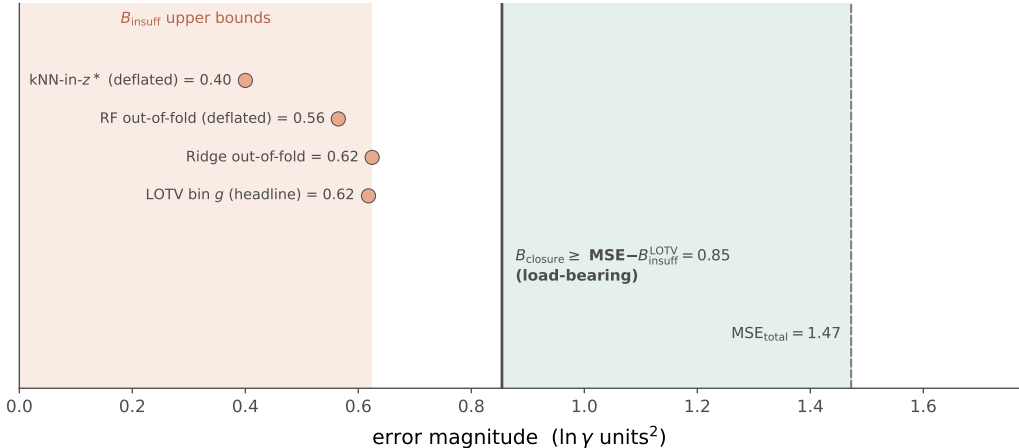
Figure 3: One-sided bounds on the closure-insufficiency split under the deployed residual-only convention. The load-bearing LOTV bound B_{\text{closure}} \geq \text{MSE} - B_{\text{insuff}}^{\text{LOTV}} \approx 0.85 ( \text{MSE} = 1.47 ) exceeds every valid B_{\text{insuff}} upper bound (salmon); the white gap is the assumption-free separation, and the teal region is the closure share it lower-bounds (deterministic on this n=60 set; its generalization is the two-way cluster-bootstrap frequency P_{\text{boot}} \approx 0.78 ). The LOTV binning bound is headlined because it conditions on the scalar g(z^*) and is immune to the near-duplicate leakage that deflates the z^* -neighbour estimators (§6.2); the constant-offset (Jensen) bound inverts here (App. C).
