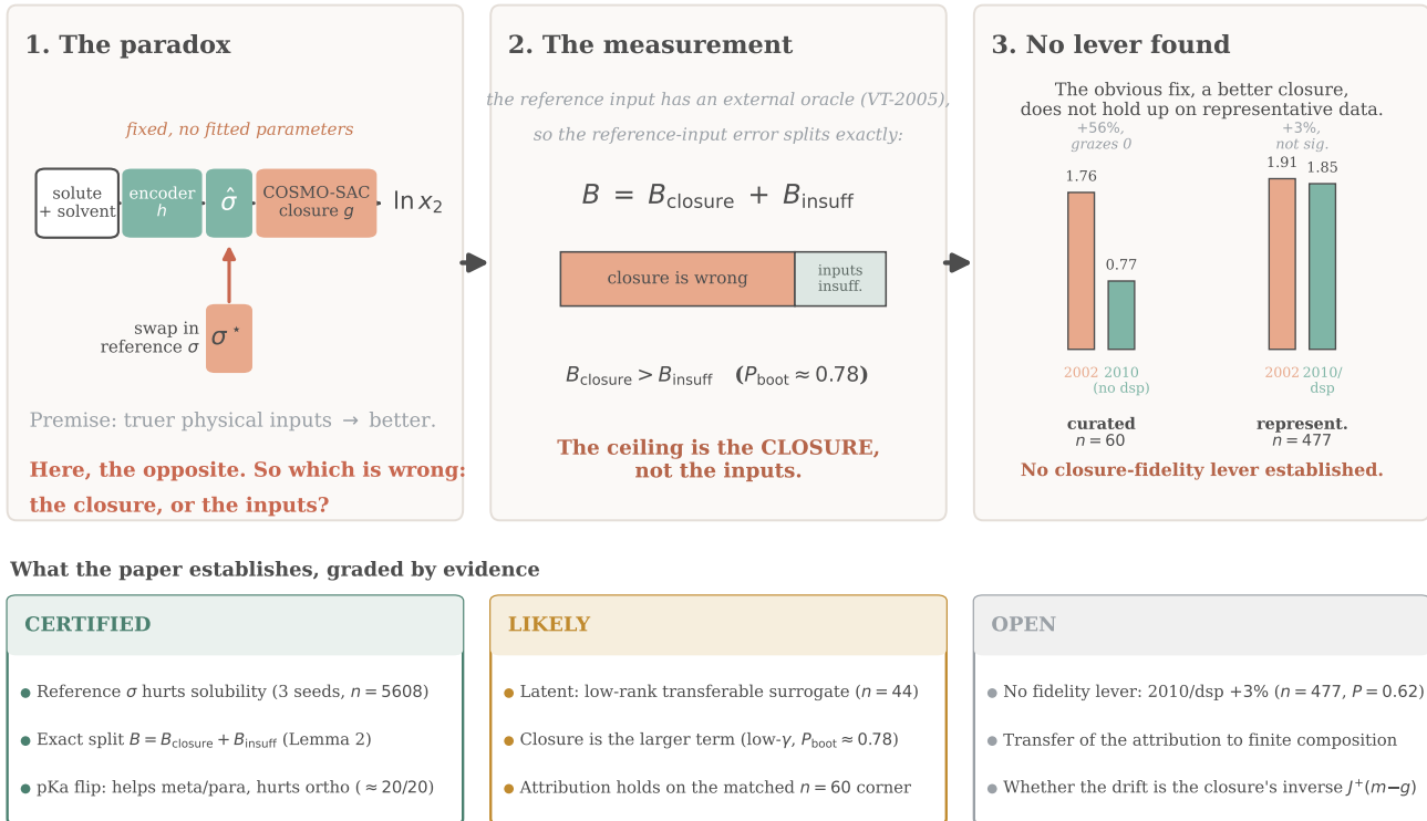
Figure 1: The paper in one view. A learned encoder h predicts a physical latent—a molecular \sigma -profile—that a fixed COSMO-SAC closure g (no fitted parameters) turns into a solubility. (1) The paradox : replacing the learned \hat{\sigma} with the external quantum-chemical reference \sigma^* (VT-2005) makes the prediction worse than a free learned head—so which is wrong, the closure or the inputs? (2) The measurement : because the latent has an external oracle, the reference-input risk splits exactly into a closure-misspecification part B_{\text{closure}} and an input-insufficiency part B_{\text{insuff}} ; on the matched low- \gamma set the closure term is the larger on the bounds we can compute ( B_{\text{closure}} > B_{\text{insuff}} , likely; P_{\text{boot}} \approx 0.78 ). (3) No lever found : on representative data a fair, validated comparison of the 2002 and modern (COSMO-SAC-2010/dsp) kernels does not establish that raising closure fidelity removes the penalty—we locate the ceiling but offer no fix inside this closure family. Bottom : every claim in the paper graded by strength of evidence (certified / likely / open), with the same one-sided-bound and scope caveats made in the text.
