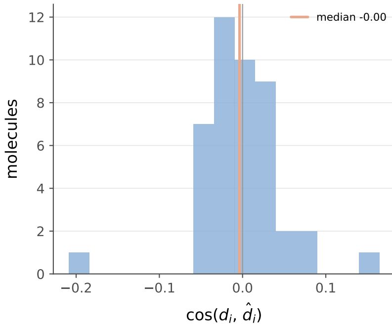
Per-molecule drift alignment
