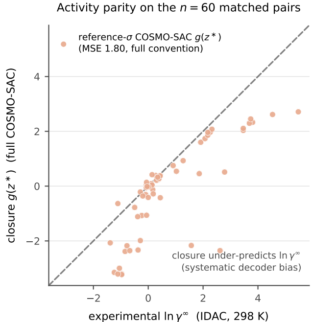
Figure S4: Activity-coefficient parity on the n=60 matched pairs. The reference- \sigma COSMO-SAC closure g(z^*) (salmon) falls below the diagonal at larger \ln \gamma_2^\infty , under-predicting the activity coefficient (MSE 1.80, full convention).
