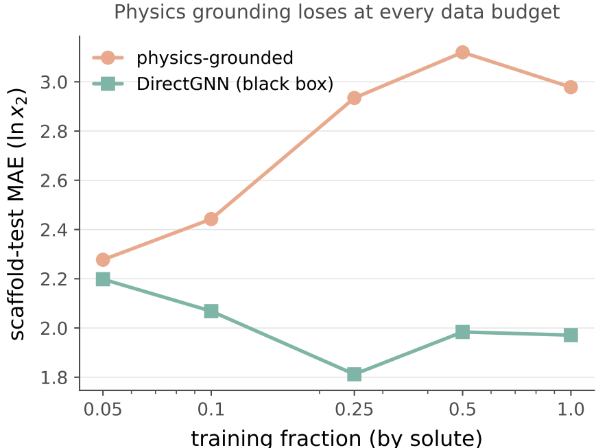
Figure 6: Data-efficiency curve. The physics-grounded arm (salmon) trails the DirectGNN black box (teal) at every training-data fraction; the gap is smallest at the least data and large thereafter—the opposite of the low-data advantage a physics prior is supposed to provide.
