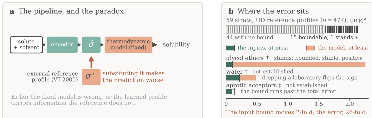
Figure 1: Overview. (a) A learned encoder predicts a charge-density profile \hat{\sigma} that a fixed thermodynamic model turns into a solubility; the arrow marks the evaluation-time substitution of the reference \sigma^* , which makes it worse. (b) The counterpart error on infinite-dilution activity data: the strip is every stratum searched, the bars the three boundable solvent classes; only the starred class stands, each mark carrying its own reason, and each block is a one-sided bound rather than an interval. Training-time supervision is not drawn.
