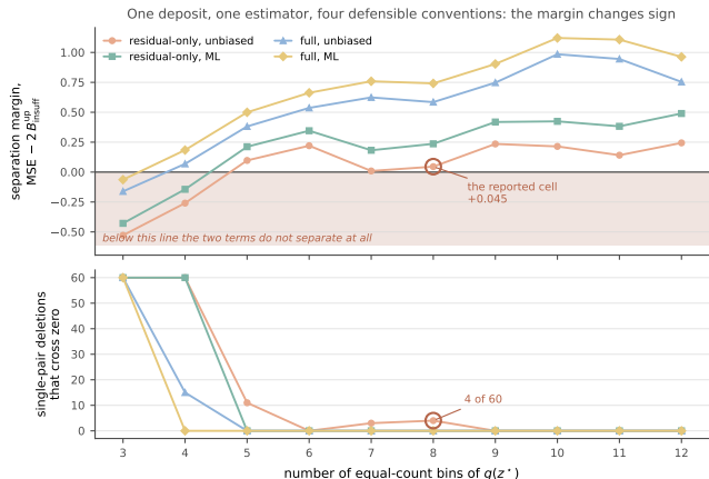
Figure 6: The same rows, the same estimator, and four defensible conventions. The VT-2005 matched set ( n = 60 ) at every bin count from three to twelve, under both within-bin variance conventions (unbiased, maximum-likelihood) and both combinatorial ones (residual-only, full). (a) the separation margin \text{MSE} - 2B_{\text{insuff}}^{\text{up}} ; below zero Lemma 1 separates nothing. (b) how many of the 60 single-pair deletions send that margin below zero. The ringed point is the cell §2.5 fixes in advance and this section reports. The aggregate spans -0.53 to +1.12 across cells that are each individually defensible, which is why the choices are fixed before the data are seen rather than justified after.
