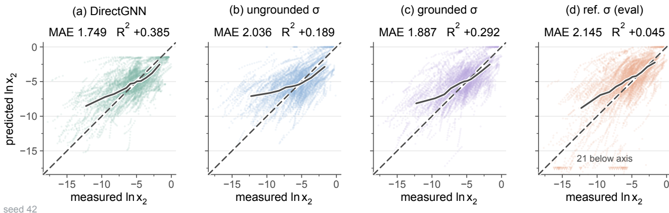
Figure S8: Solubility parity for four arms of the controlled comparison: predicted against measured \ln x_2 on the 5608 labelled test rows of the scaffold split, which are 763 solute–solvent pairs over 147 solutes and 70 solvents measured between 248 and 368 K. (a) DirectGNN, the closure-free control; (b) COSMO-SAC over an unsupervised \sigma -profile; (c) the same closure with \sigma -profile supervision during training; (d) the arm of (c) with the reference VT-2005 profile substituted at evaluation. Dashed, the identity. Solid, the median prediction in twelve equal-count bins of the measurement. Each panel header carries that panel’s own MAE and R^2 . Both axes span the measured range with a margin around it, and the markers along the foot of (d) are its 21 predictions that fall below the frame, each at its own measured value. Panels (b), (c) and (d) come from the five-seed leak-free re-run: the ungrounded, grounded and \sigma -oracle \sigma arms respectively.
