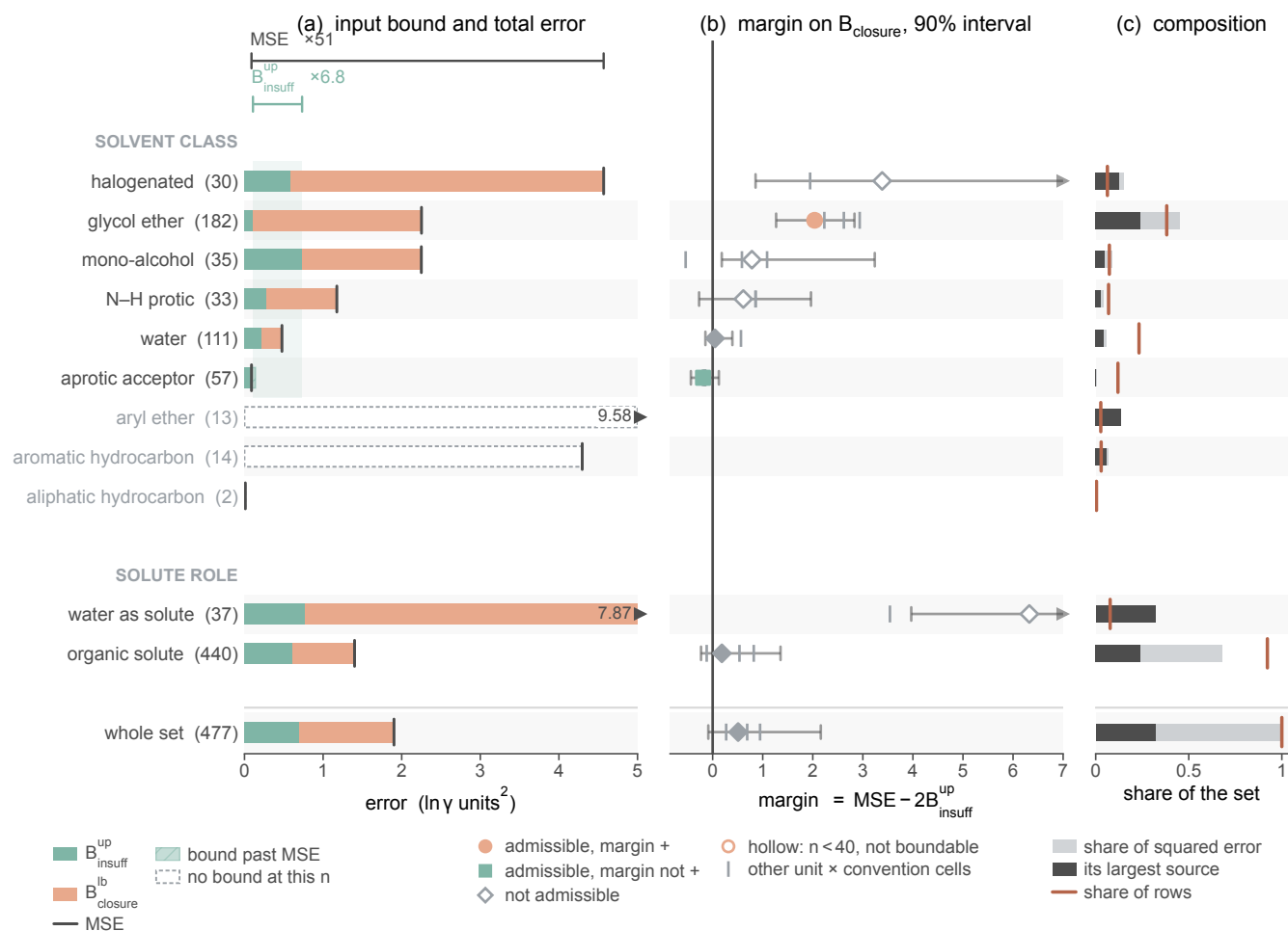
Figure S3: Where the closure binds, and where the two terms do not separate , by solvent class and by solute role, on the broad IDAC set (477 rows, 185 pairs, 78 solutes, 36 solvents, 15 source publications). Bars, points and shares are at the row unit under the residual-only convention, at one estimator cell for every stratum—eight equal-count bins of g(z^*) with the unbiased within-bin variance. (a) each stratum's input-insufficiency bound and its total error; (b) the margin between them with its 90% two-way cluster-bootstrap interval, the other three unit \times convention cells as grey ticks; (c) each stratum's share of the set's squared error, the part carried by its largest source publication drawn dark. Twelve cells at the granularity reported here, drawn from the 59-stratum map of Tables S12–S15. Strata on the two axes overlap, so panel (c)'s shares do not sum down the column.
