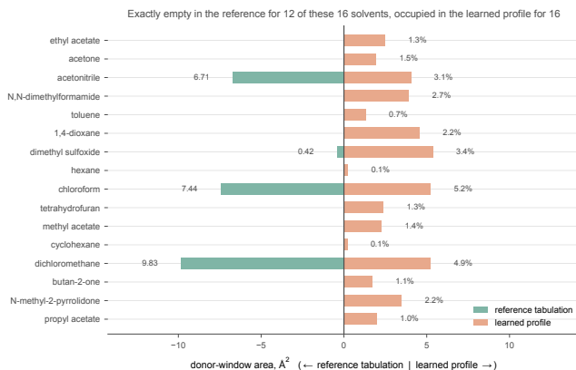
Figure S9: The window the hydrogen-bond term reads, in the reference tabulation and in the learned profile. The sixteen solvents carrying the most scored rows, ordered by that count. Left of the axis, the reference tabulation’s donor-window area, which is exactly 0.000 \text{ \AA}^2 in twelve of them and is drawn with its value where it is not; right of the axis, the learned profile’s area in the same window, annotated with the fraction of that molecule’s total surface. Both halves are on one scale. The learned areas are seed-averaged over the grounded arms of Fig. 2, seeds 42 to 46, so the figure prices the arms the substitution contrast rests on. The reference is empty in twelve of the sixteen and the learned profile is occupied in all sixteen, while over the thirty-one scored solvents the two rank together at \rho = +0.65 : the window’s ordering is learned and its floor is not.
