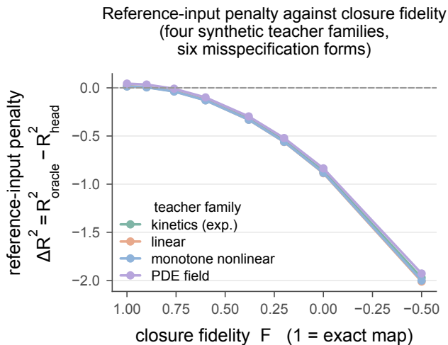
Figure S12: Closure-fidelity sweep on synthetic, non-chemical teacher functions. As the closure is made more misspecified (fidelity F falling from 1; axis reversed), the reference-input penalty \Delta R^2 = R^2_{\text{oracle}} - R^2_{\text{head}} falls monotonically below zero. Each curve is one of four teacher families, averaged over six misspecification forms, which the panel does not resolve; the four curves are visually coincident. No point is marked for the real closure.
