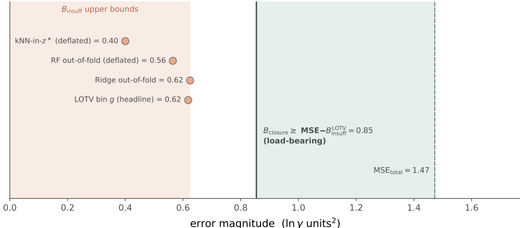
Figure 3: One-sided bounds on the closure-insufficiency split under the deployed residual-only COSMO-SAC convention—the configuration the model actually runs. The load-bearing, convention-independent bound B_{\text{closure}} \geq \text{MSE} - B_{\text{insuff}}^{\text{LOTV}} \approx 0.85 exceeds every valid B_{\text{insuff}} upper bound (salmon region); the white gap is a separation that needs no smoothness assumption, and the teal region is the closure share of the total error lower-bounded by that margin (deterministic on this n=60 set; its generalization is the two-way cluster-bootstrap frequency P_{\text{boot}} \approx 0.78 ) ( \text{MSE} = 1.47 ). We headline the law-of-total-variance (LOTV) binning bound because it conditions on the scalar g(z^*) and is immune to the near-duplicate leakage that deflates the z^* -neighbour estimators ( k -NN, RF; §6.2). The convention-specific constant-offset (Jensen) bound inverts under this deployed convention; its numbers are reported with the convention hedge in App. C.
