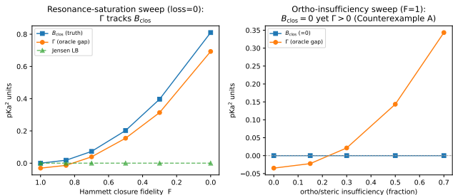
Figure 9: The diagnostic transfers to a second real closure (pKa through a Hammett LFER), on a controlled construction with known ground-truth channels. Left: varying closure fidelity with a sufficient intermediate, the grounding gap \Gamma tracks the closure bias B_{\text{closure}} (the assumption-light Jensen bound is flat here because the misspecification carries no mean offset). Right: varying an ortho/steric insufficiency channel with a well-specified closure, B_{\text{closure}} = 0 throughout while \Gamma > 0 grows—the pKa realization of the two-cause conflation of §4.3, and the reason certification rests on the decomposition, not on \Gamma .
